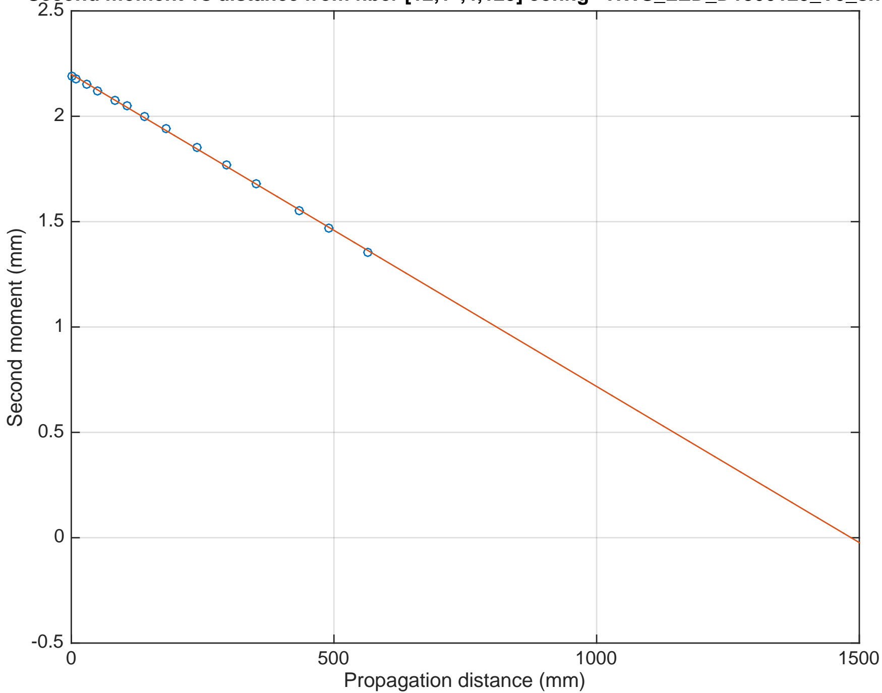
Second moment vs distance from fiber [12,1",4,125] config - HWS_LED_D1800125_V5_sn01
