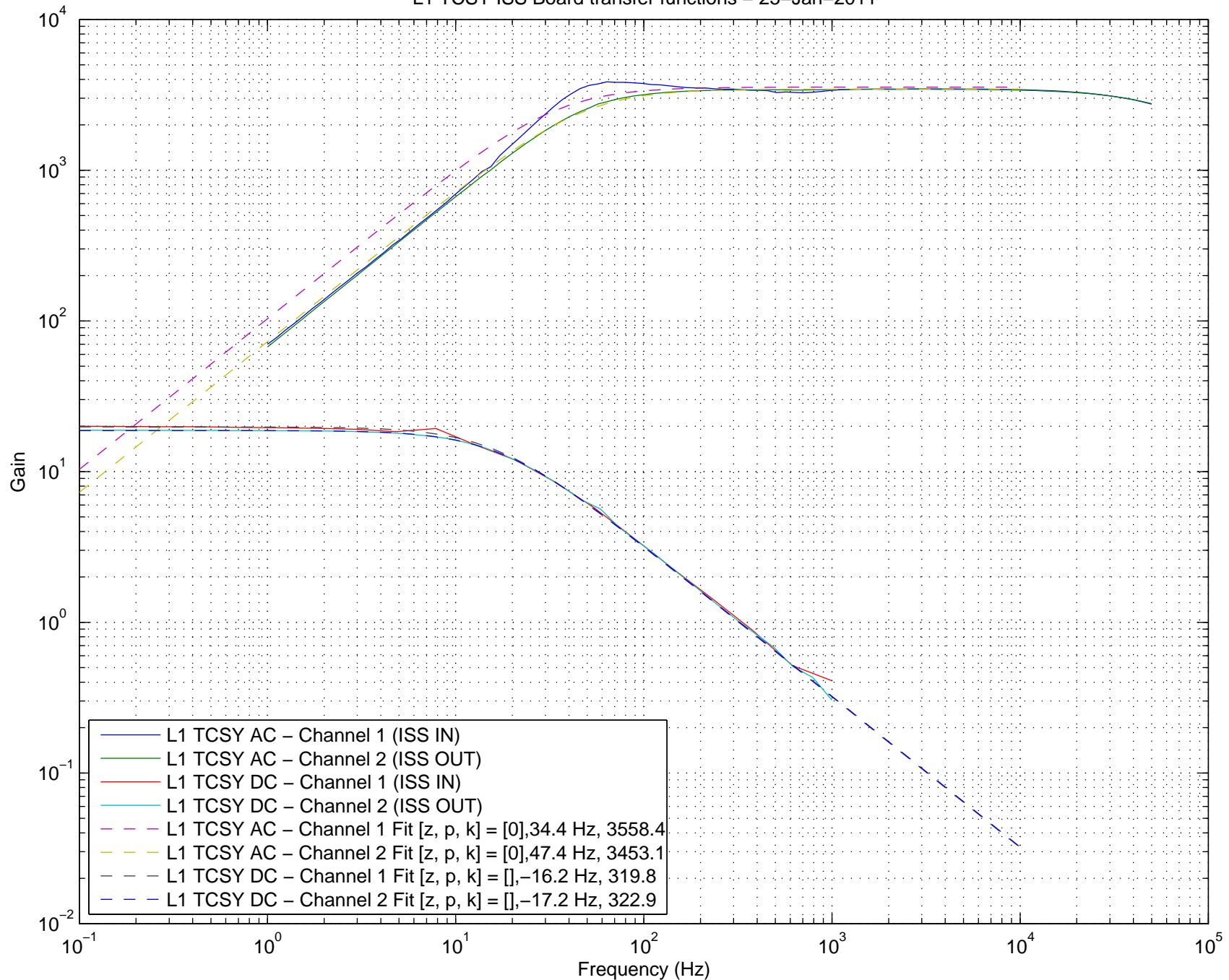
L1 TCSY ISS Board transfer functions – 25-Jan-2011
