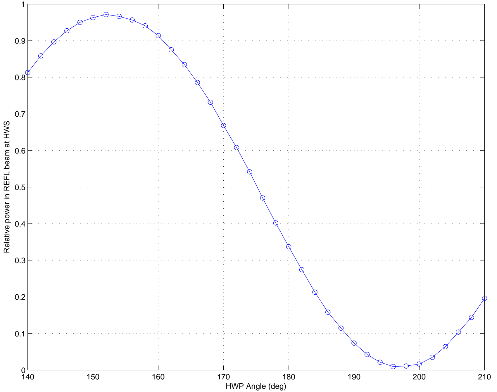
The power in the REFL relative to the total power at the HWS
