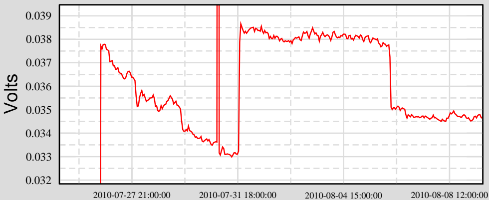
SLED On-board photo-diode voltage
