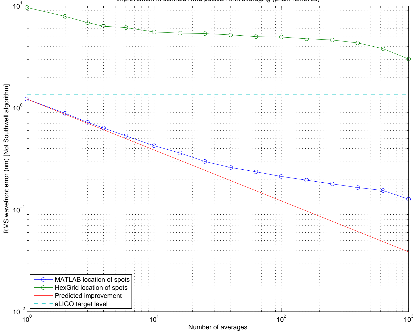
Improvement in centroid RMS position with averaging (prism removed)
