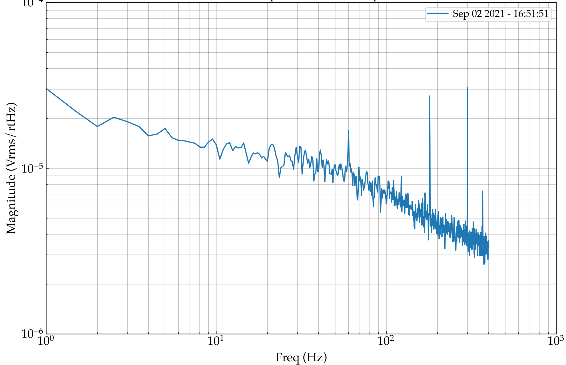
1.4 \mu\text{m} ECDL RIN Power spectrum (0 dB) - Sep 02 2021 - 16:52:59
