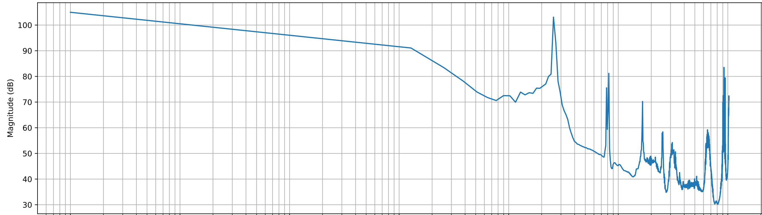
SR785 OLTF DOPO + SR560 lock () - Feb 17 2021 - 16:48:08
