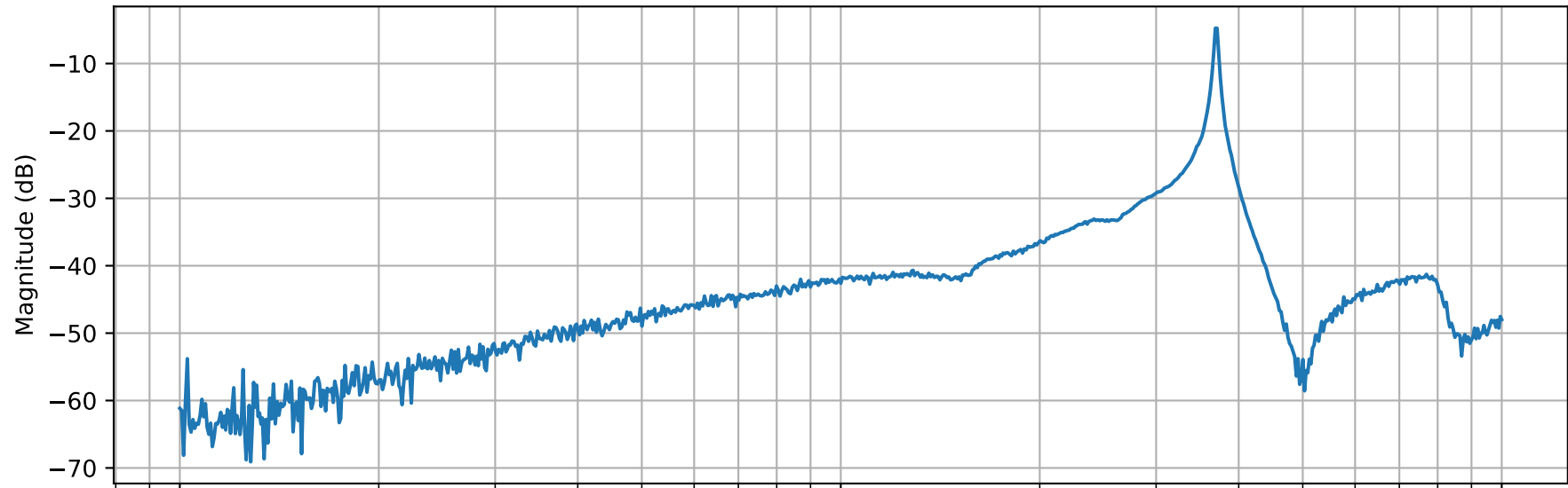
EOM Driver Transfer Function from input to RF Mon - Dec 03 2020 - 12:10:23
