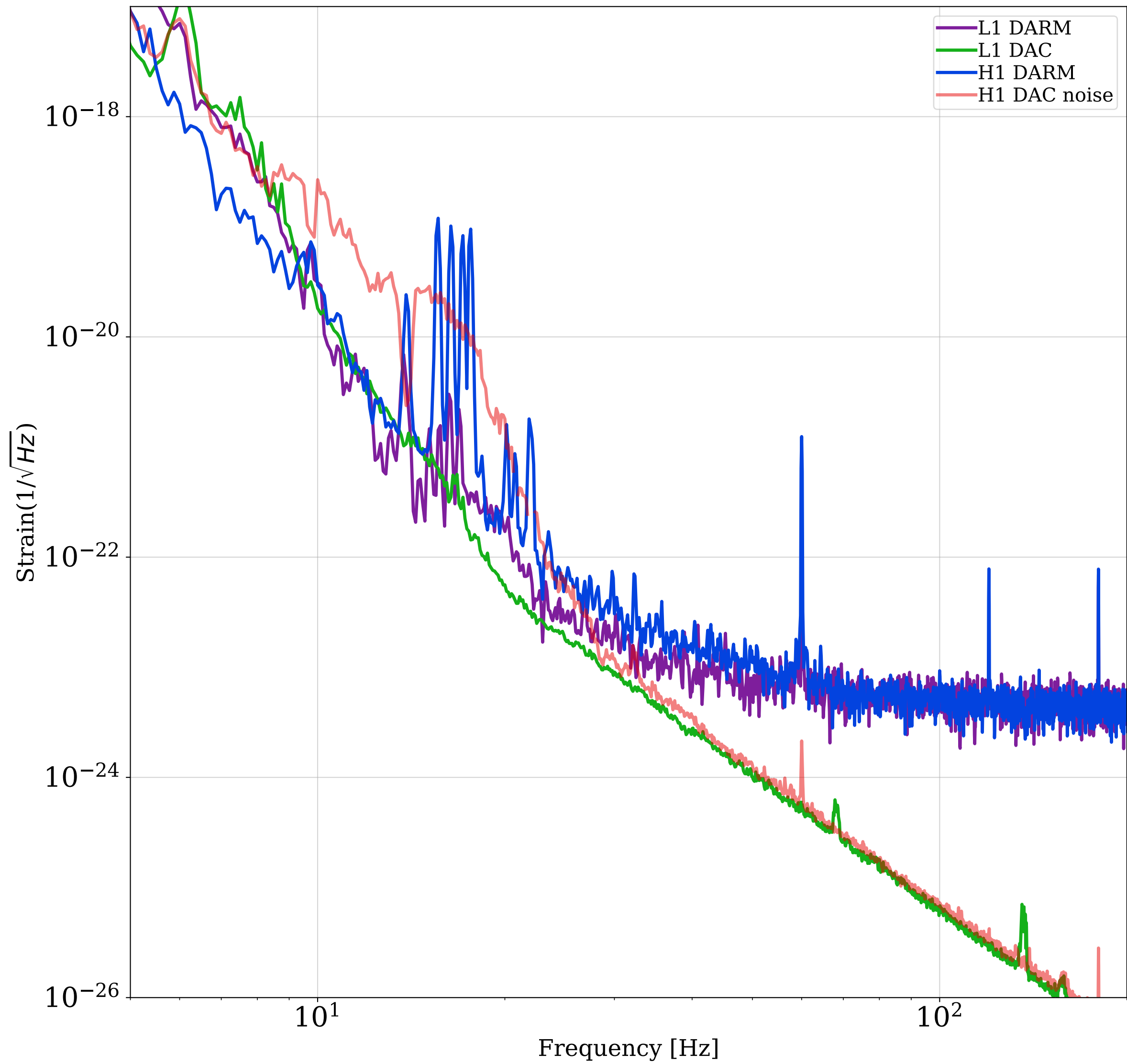
DARM NOISE vs. DAC NOISE
