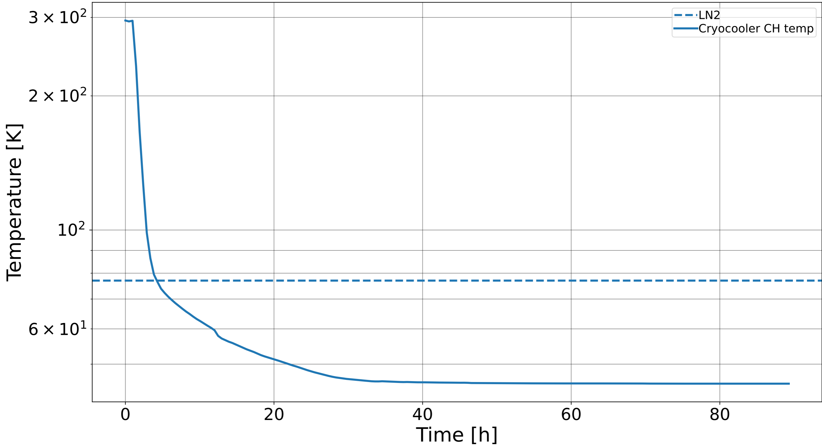
Cold head T vs LN2
