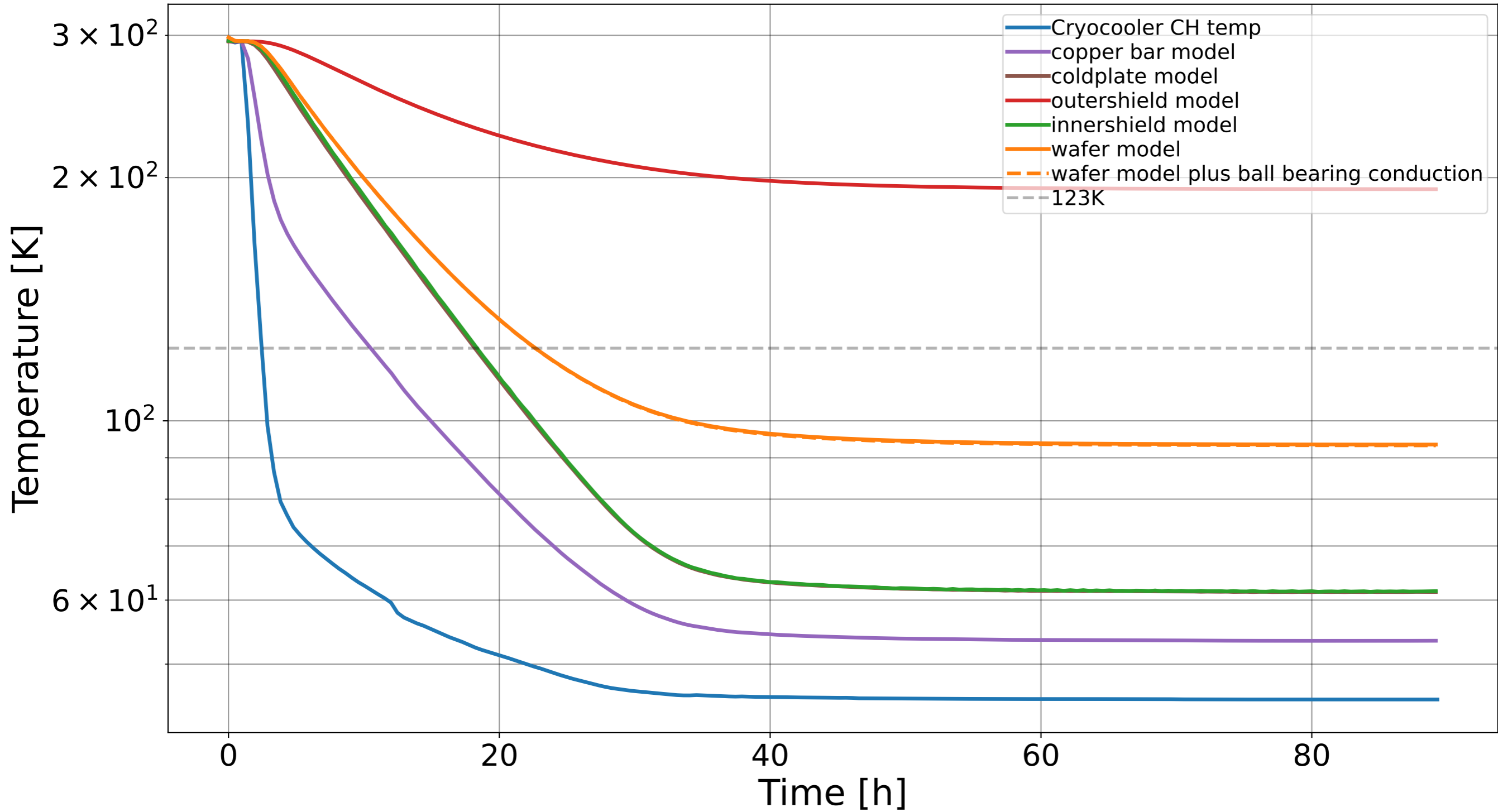
Wafercooldown model
