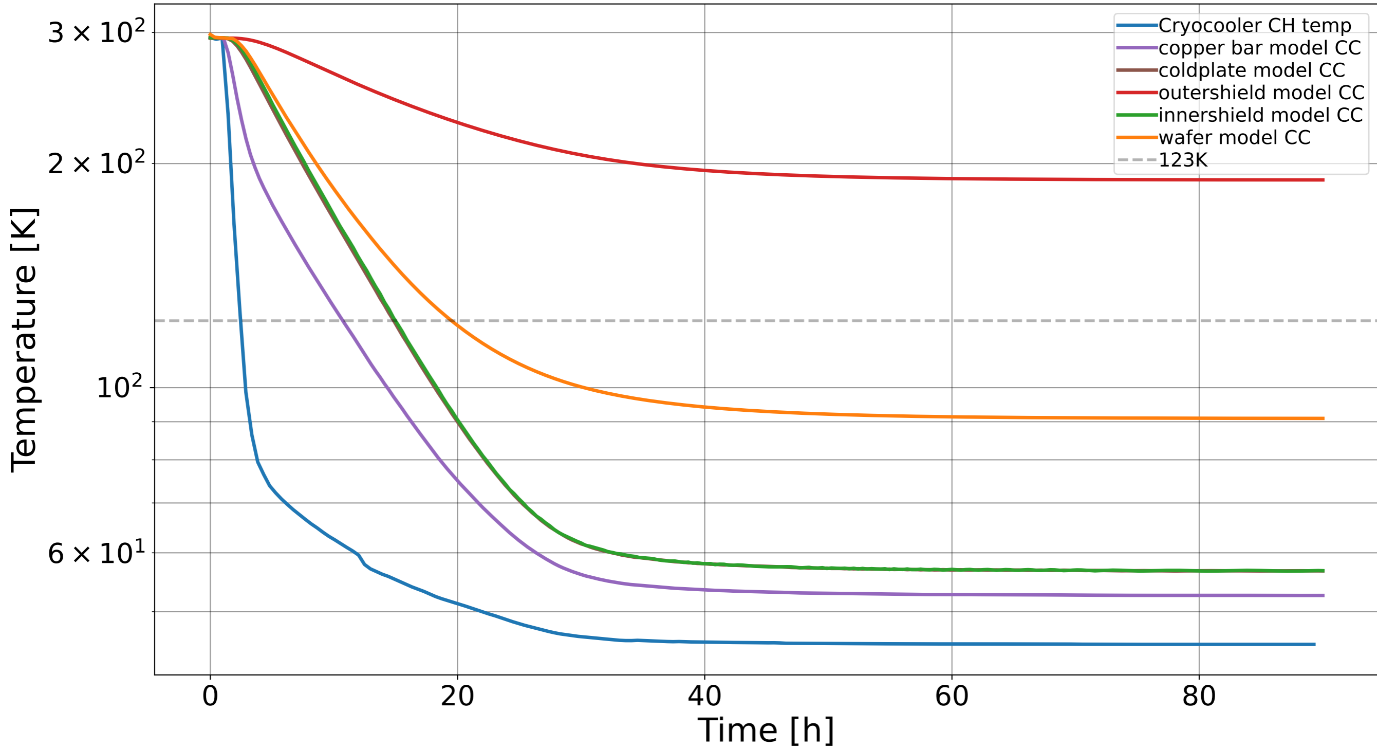
Wafercooldown model
