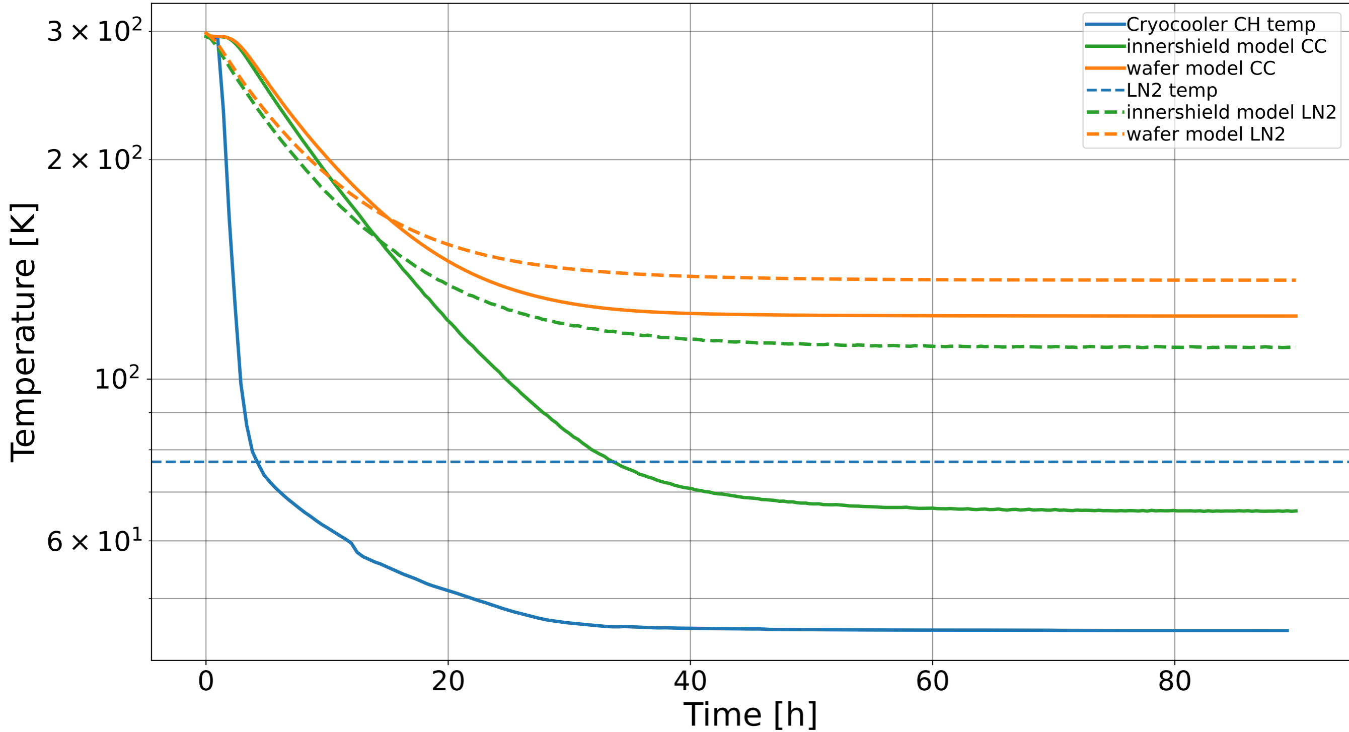
Cryocooler vs. LN2 for 2" wafer cooldown
