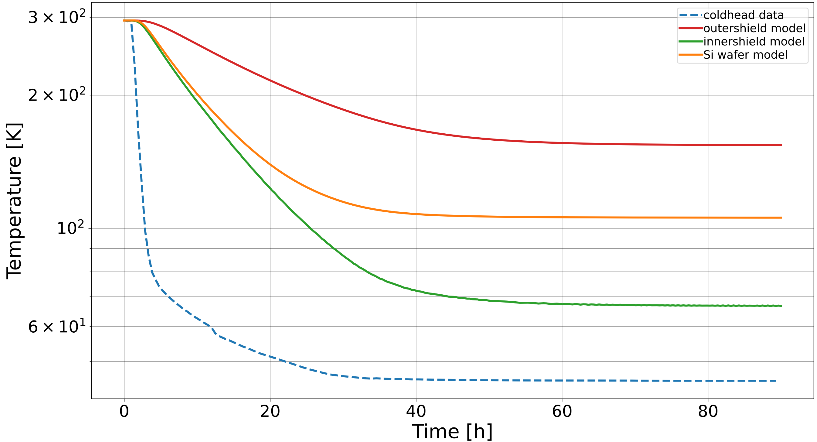
Si wafer cooldown model, Megastat
