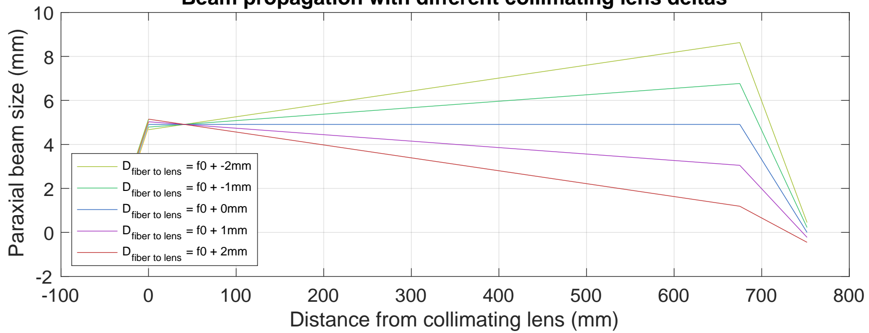
Beam radius at JPL PD with different collimating lens distances
