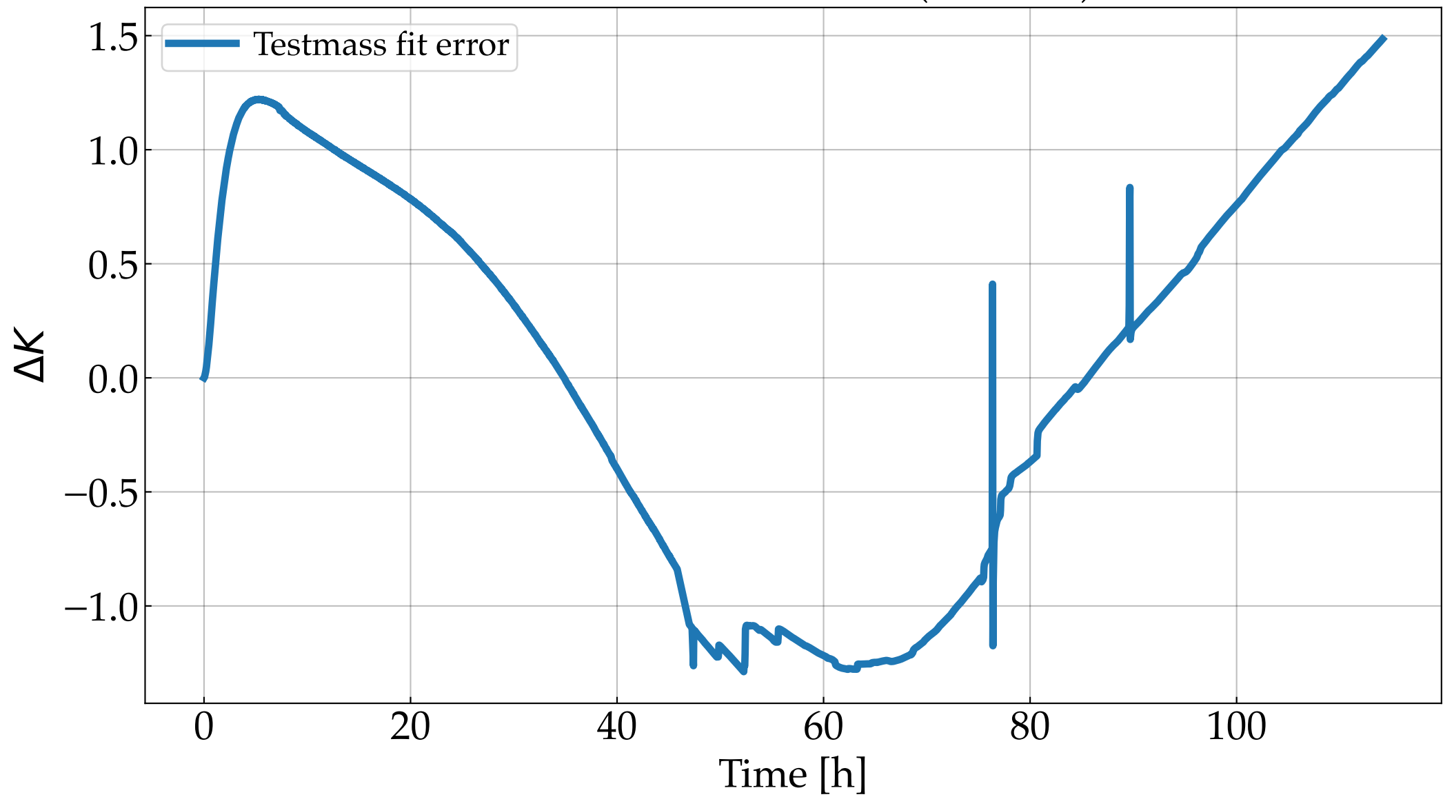
Cooldown model error (fit - data)
