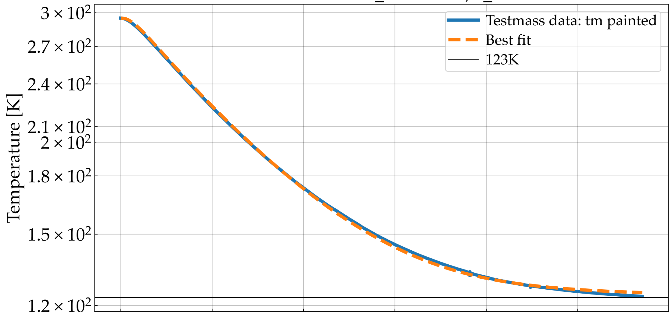
Cooldown model fit: e_{tm} = 0.597 , e_{is} = 0.202
