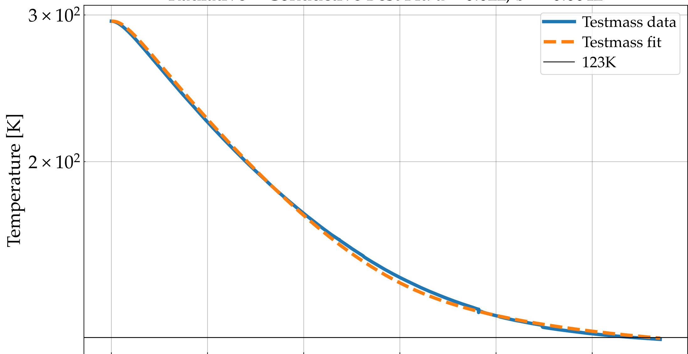
Radiative + Conductive Best Fit: a = 0.022 , b = -0.0042
