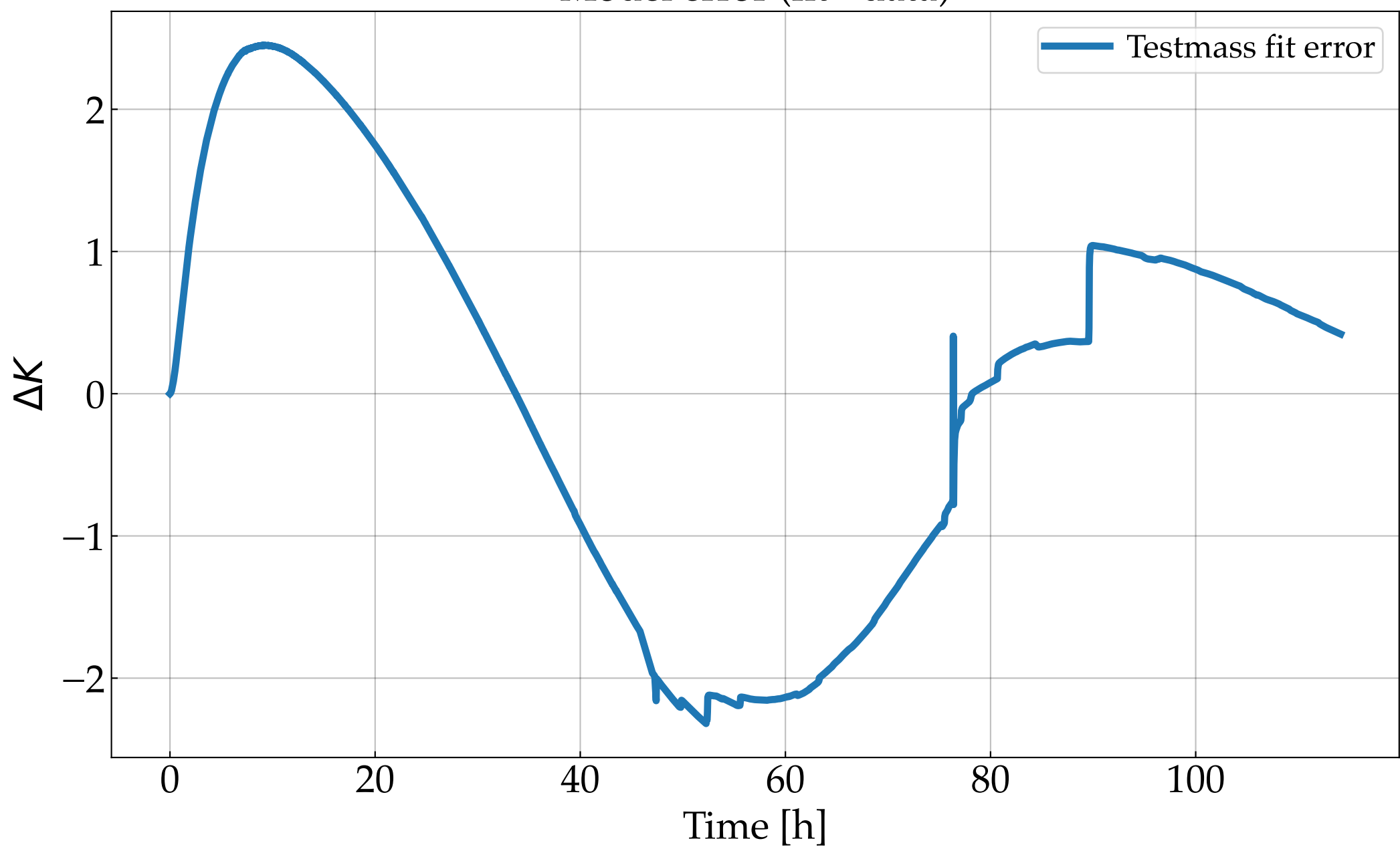
Model error (fit - data)
