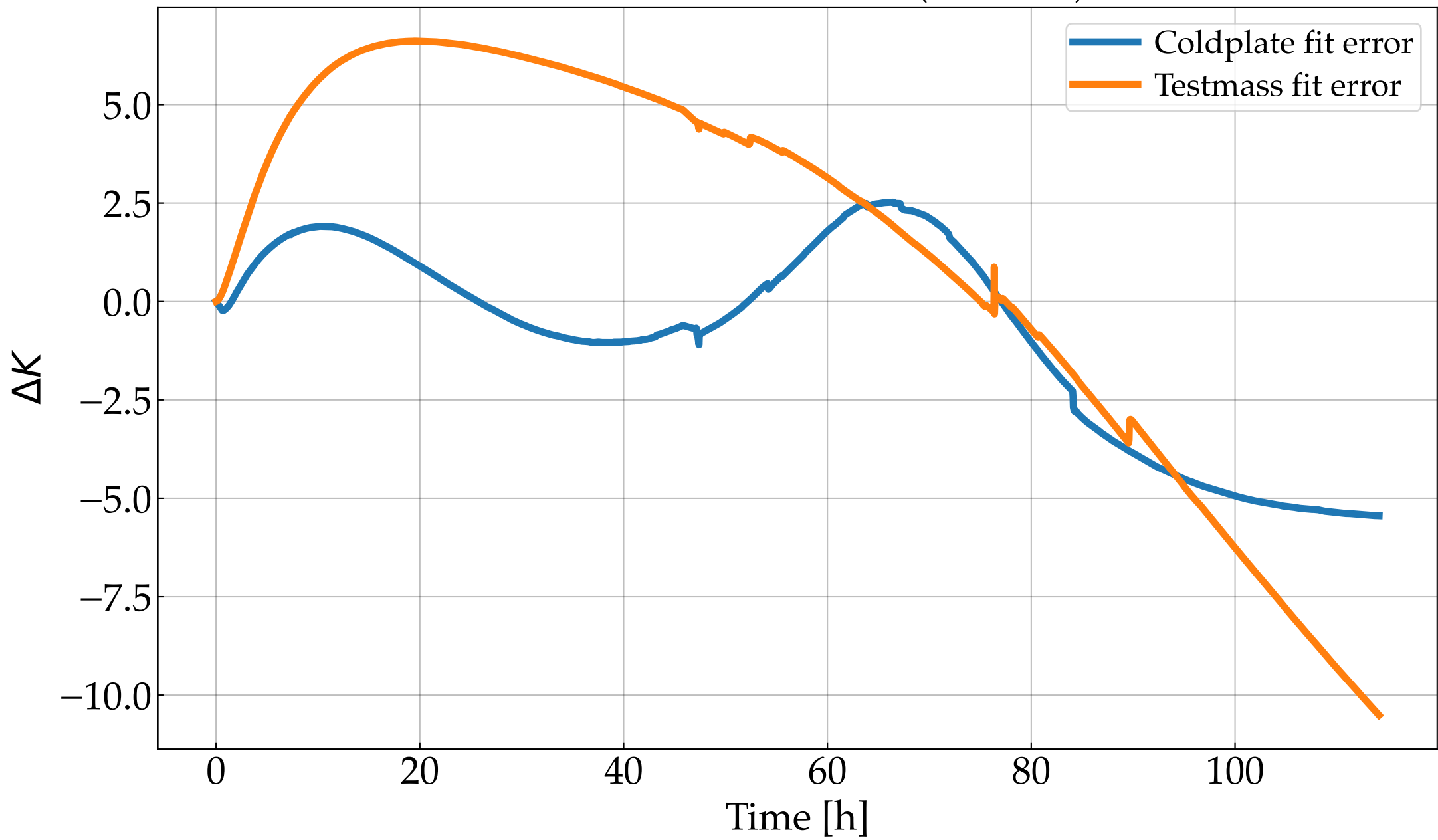
Cooldown model error (fit - data)
