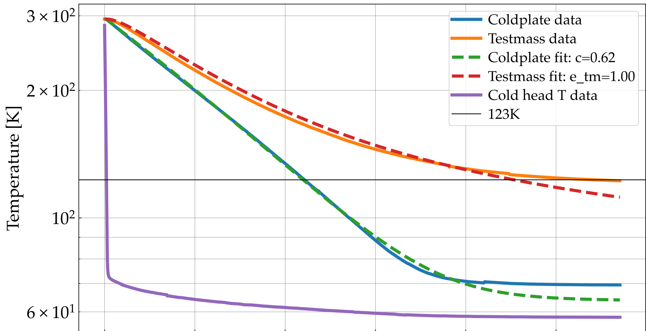
Cooldown model fit
