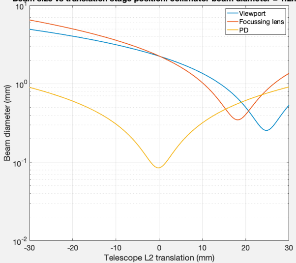
Beam size vs translation stage position: collimator beam diameter = 1.2mm
