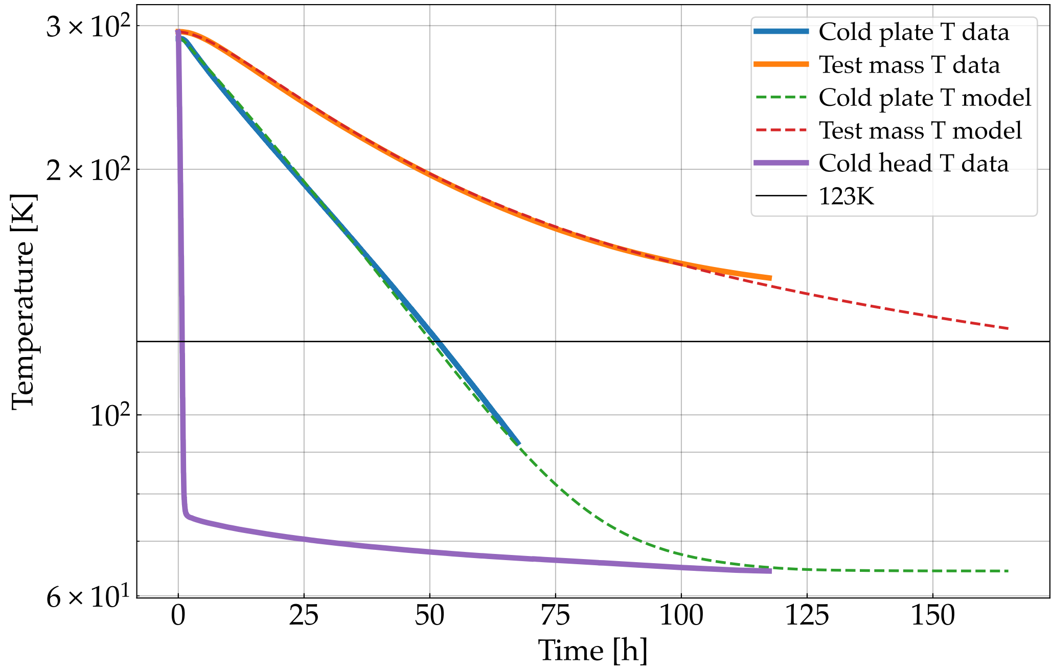
Cooldown with uncoated test mass
