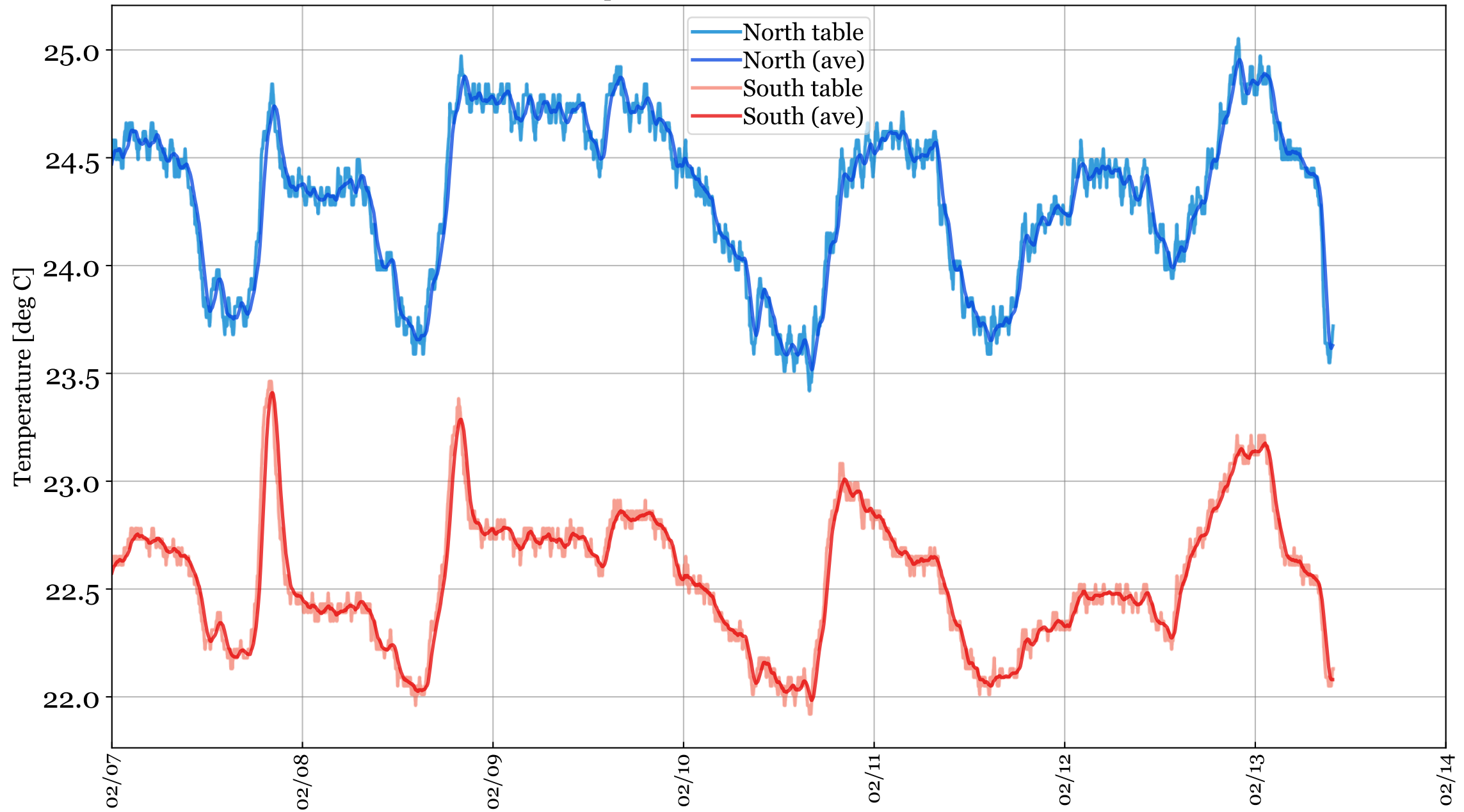
Temperature Fluctuations in QIL (B265B)
