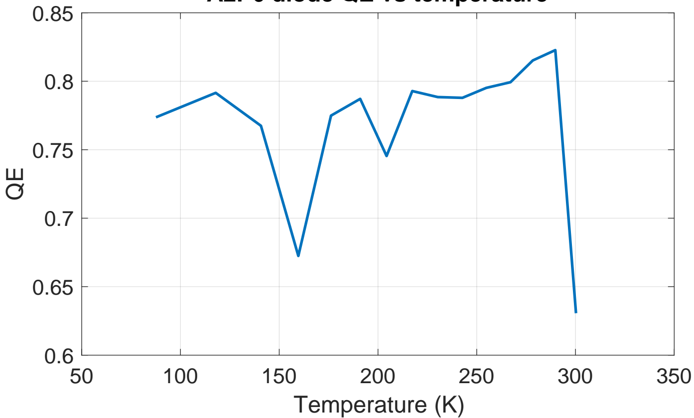
A2P6 diode QE vs temperature
