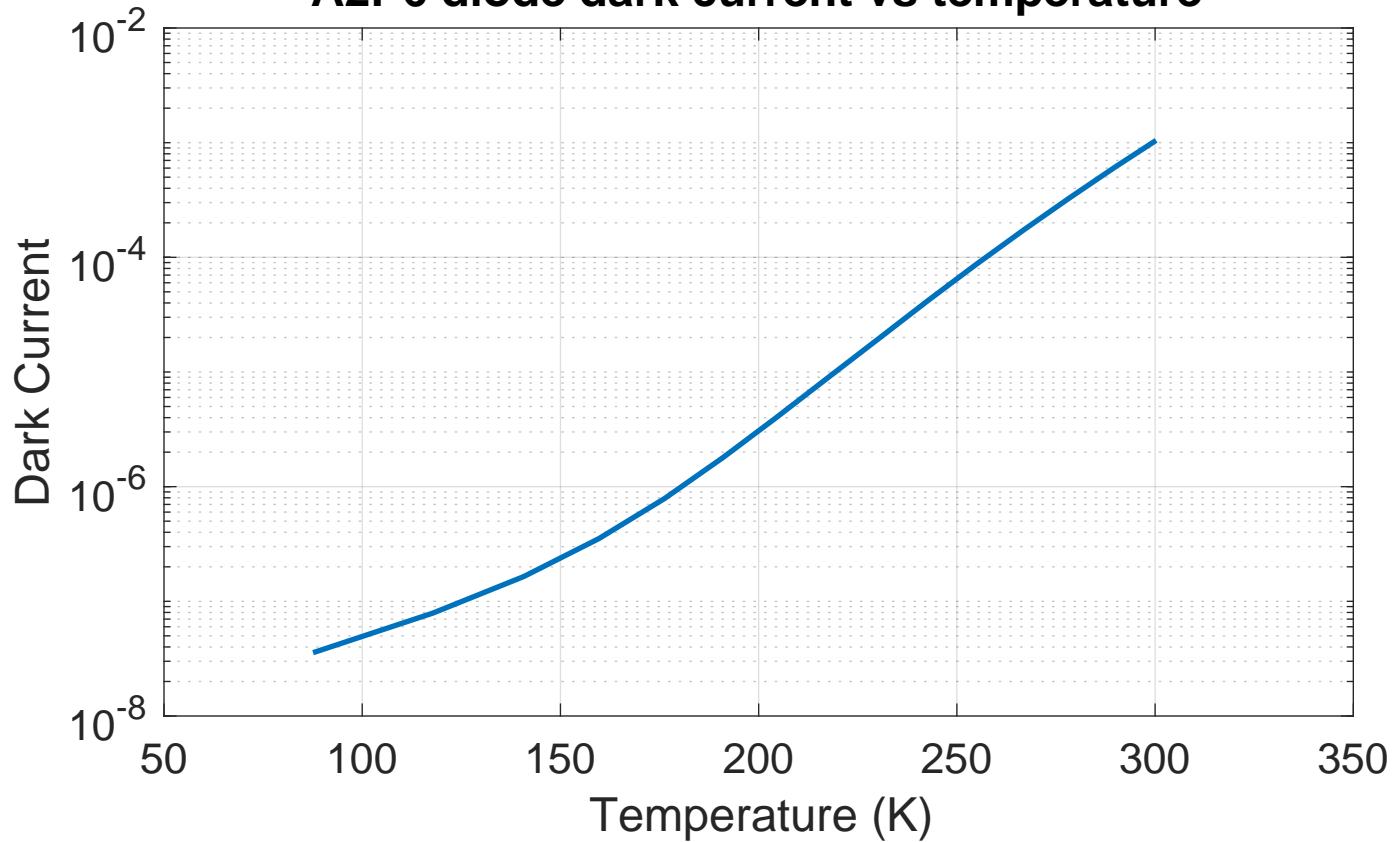
A2P6 diode dark current vs temperature
