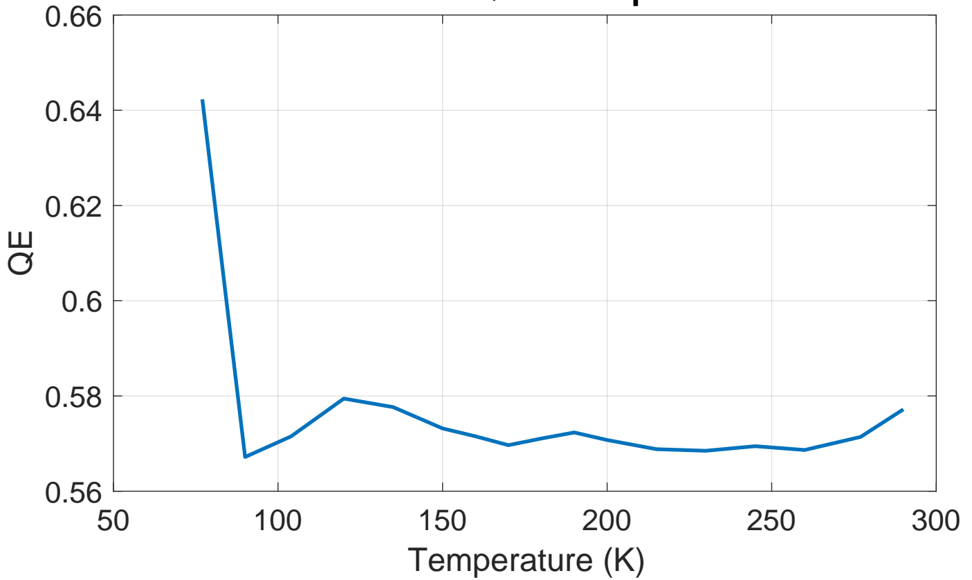
A2P2 diode QE vs temperature
