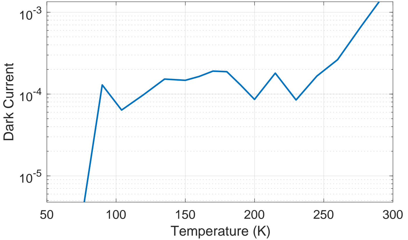
A2P2 diode dark current vs temperature
