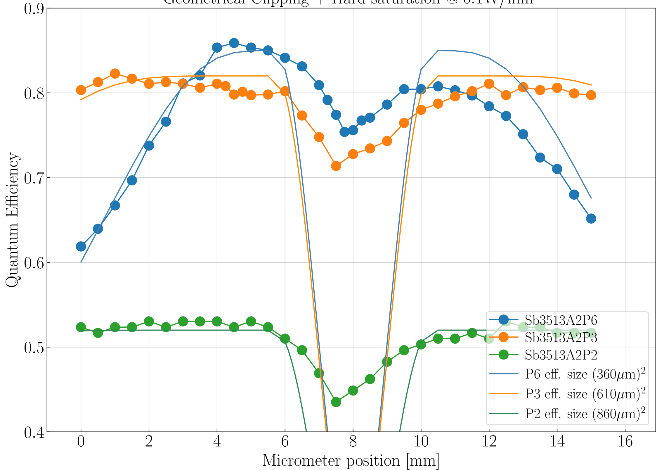
Geometrical Clipping + Hard saturation @ 0.1W/mm 2
