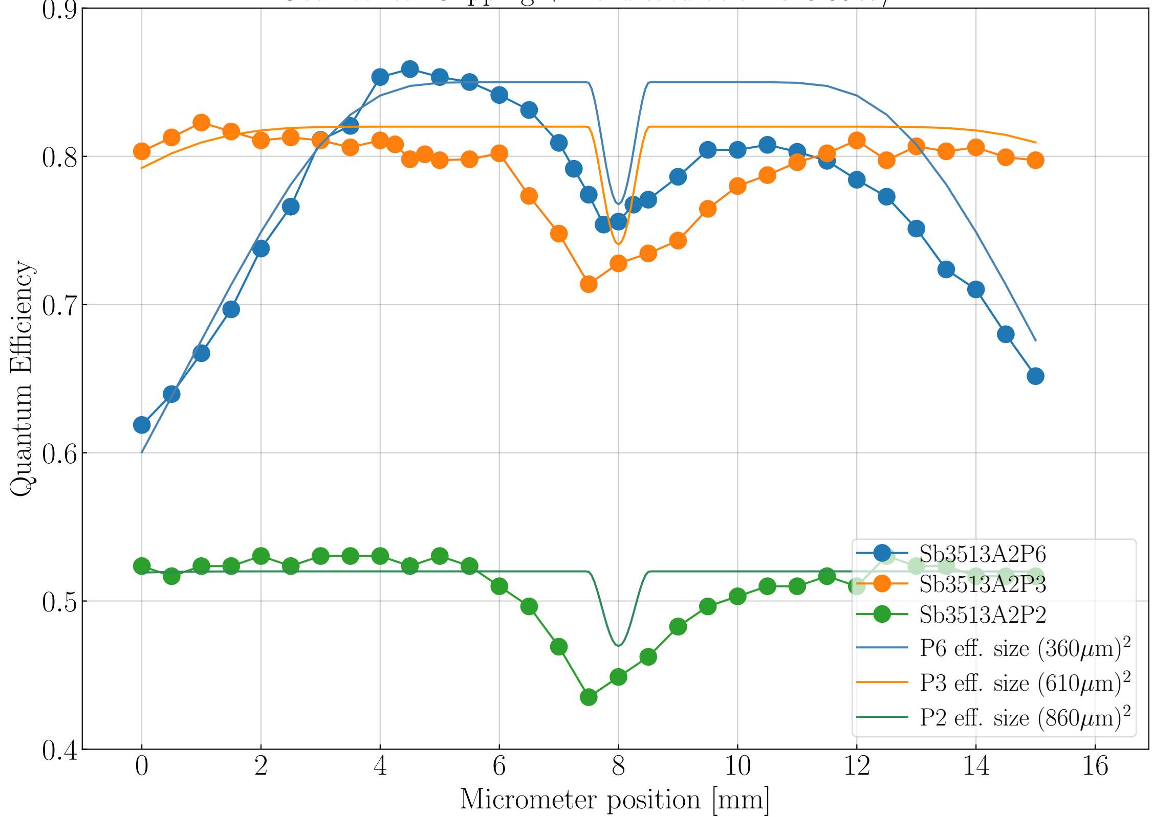
Geometrical Clipping + Hard saturation @ 0.85W/mm 2
