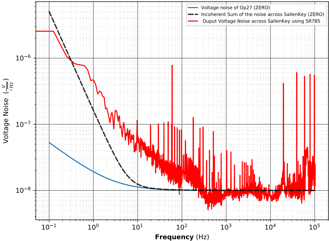
Sallen Key filter output voltage noise
