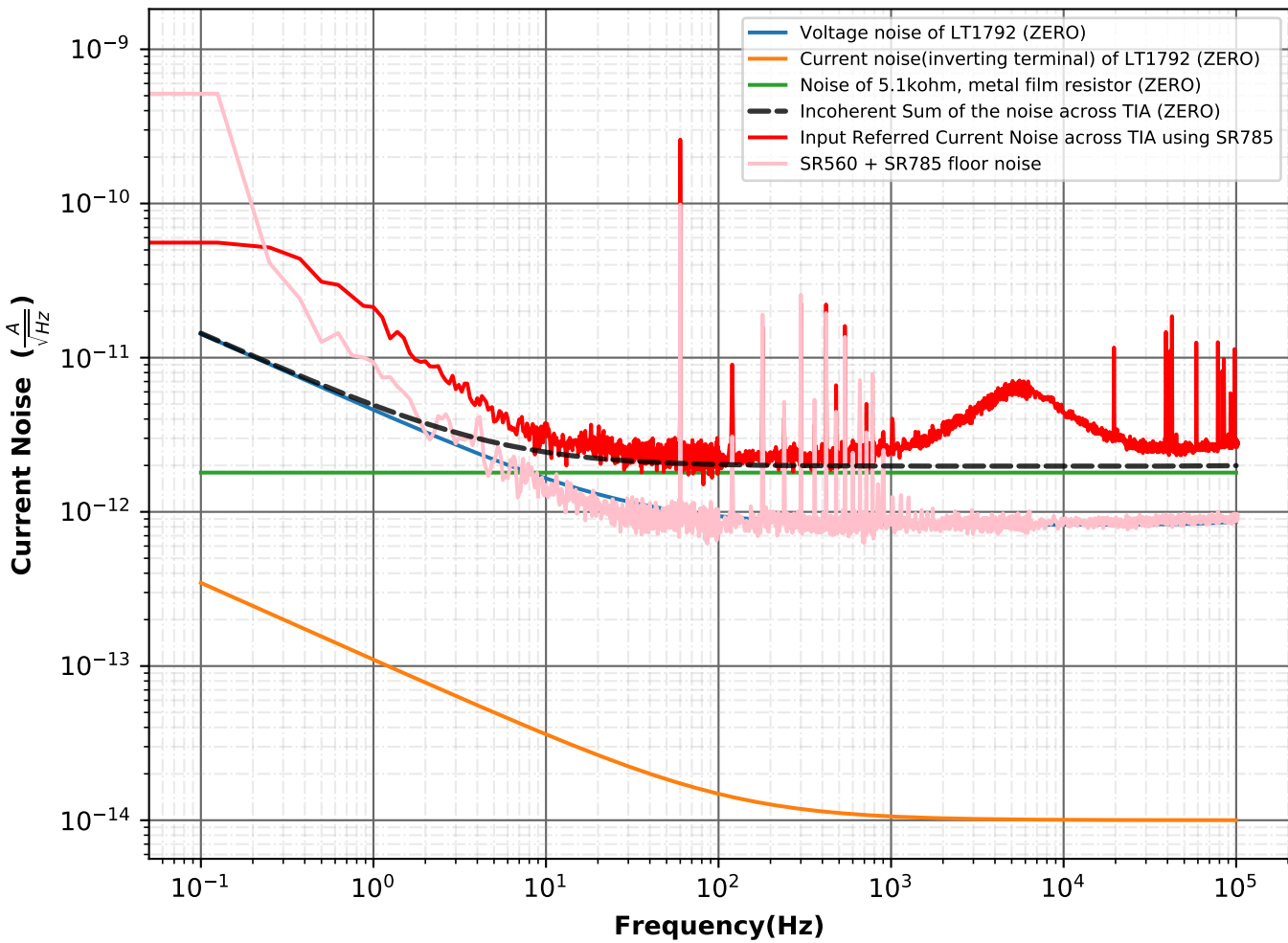
Input Referred Current Noise across transimpedance amplifier using LT1792
