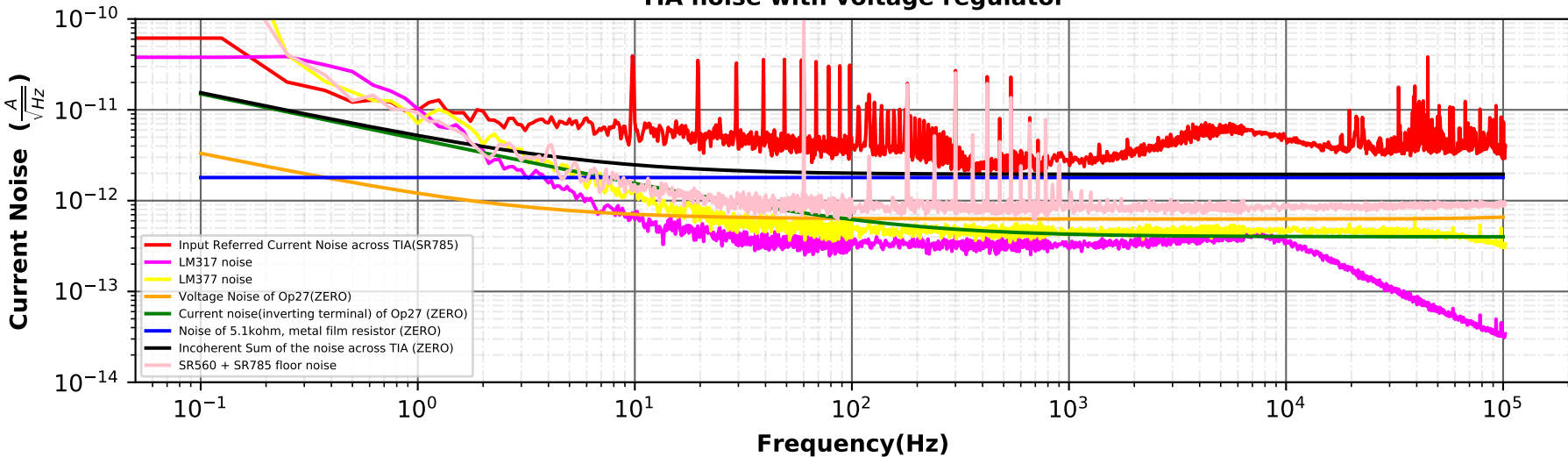
TIA noise with voltage regulator
