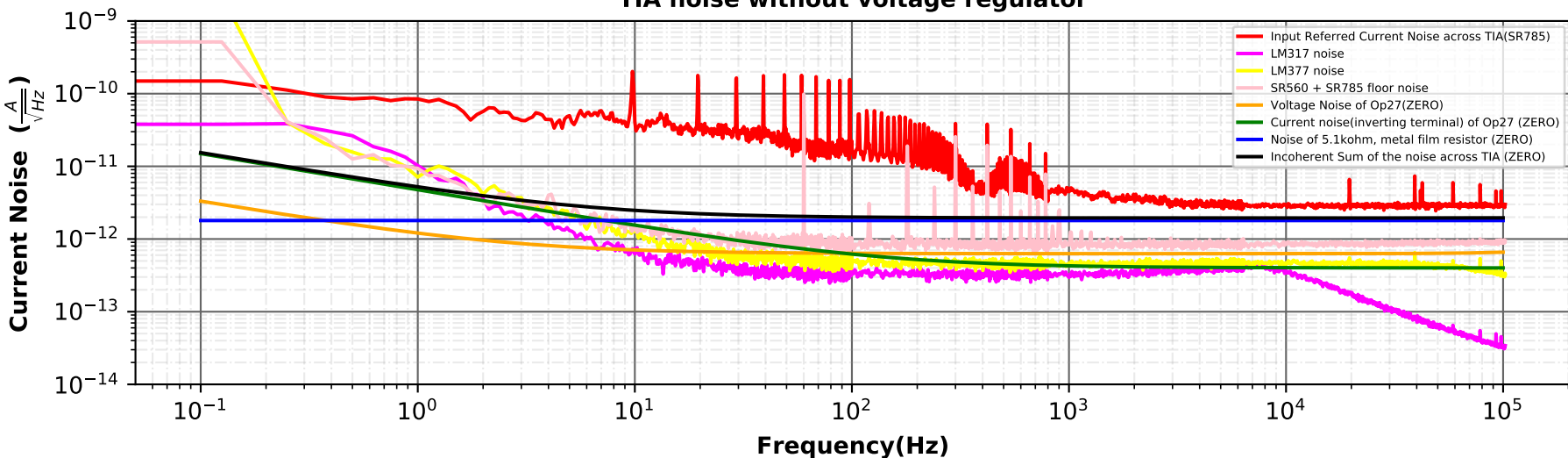
TIA noise without voltage regulator
