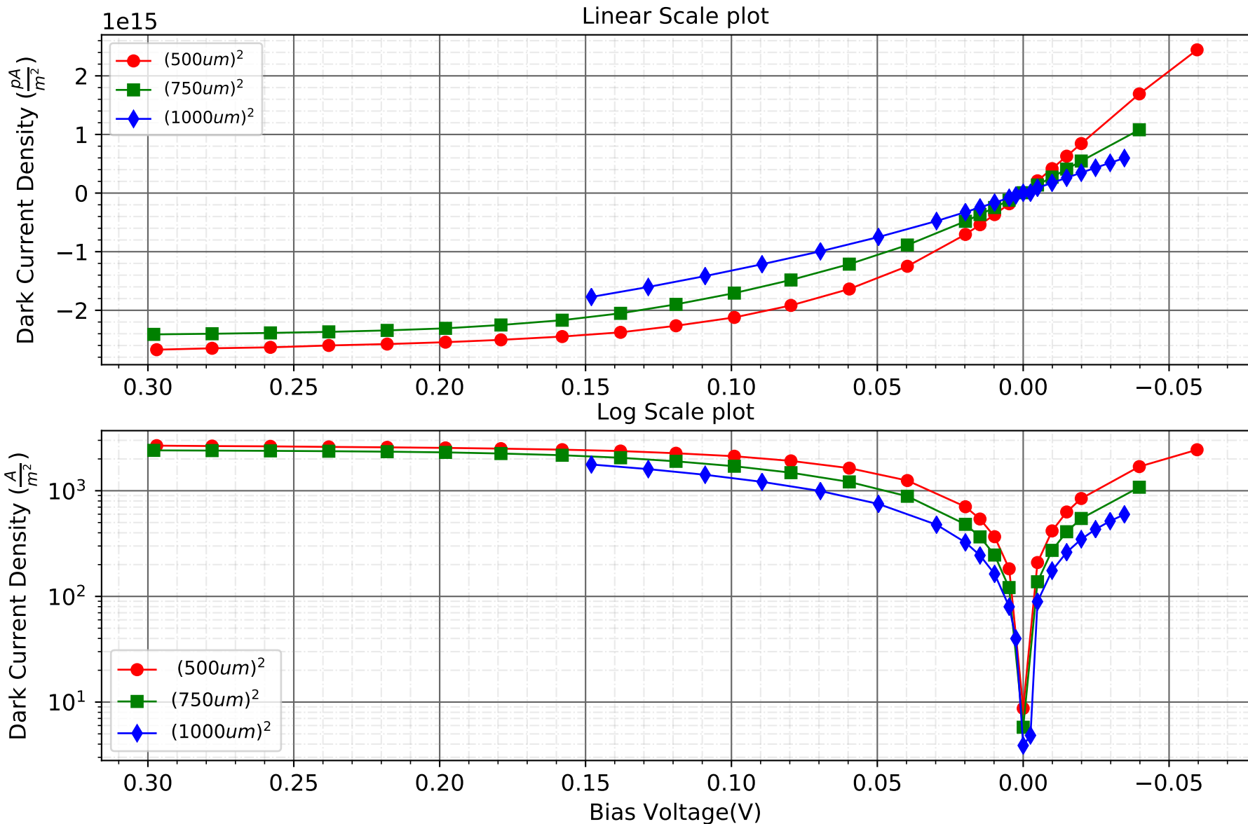
Dark Current Density across Sb3513_A2 for different bias voltage
