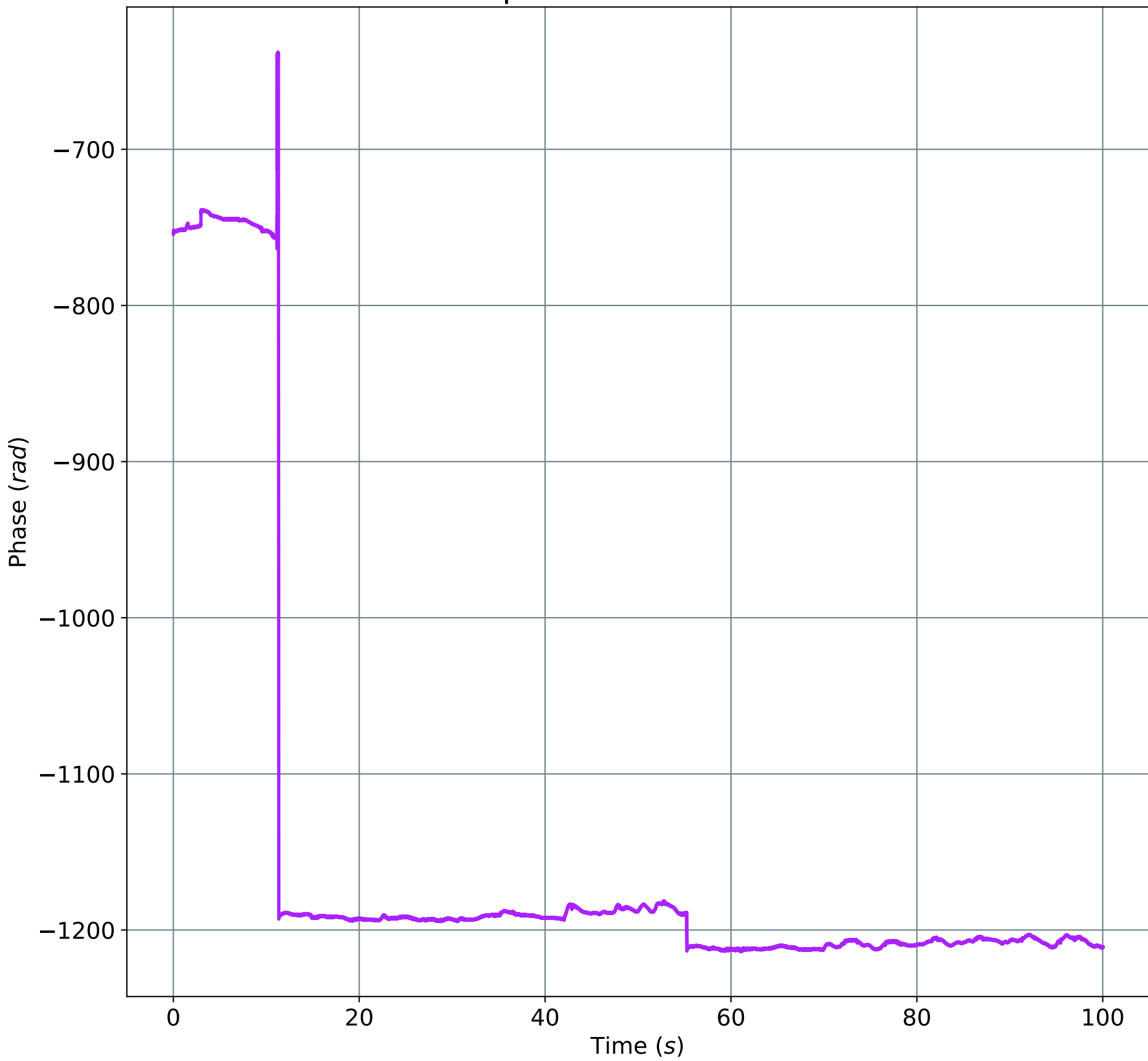
Phase of 2 \mu m Mach Zehnder IFO Arm
