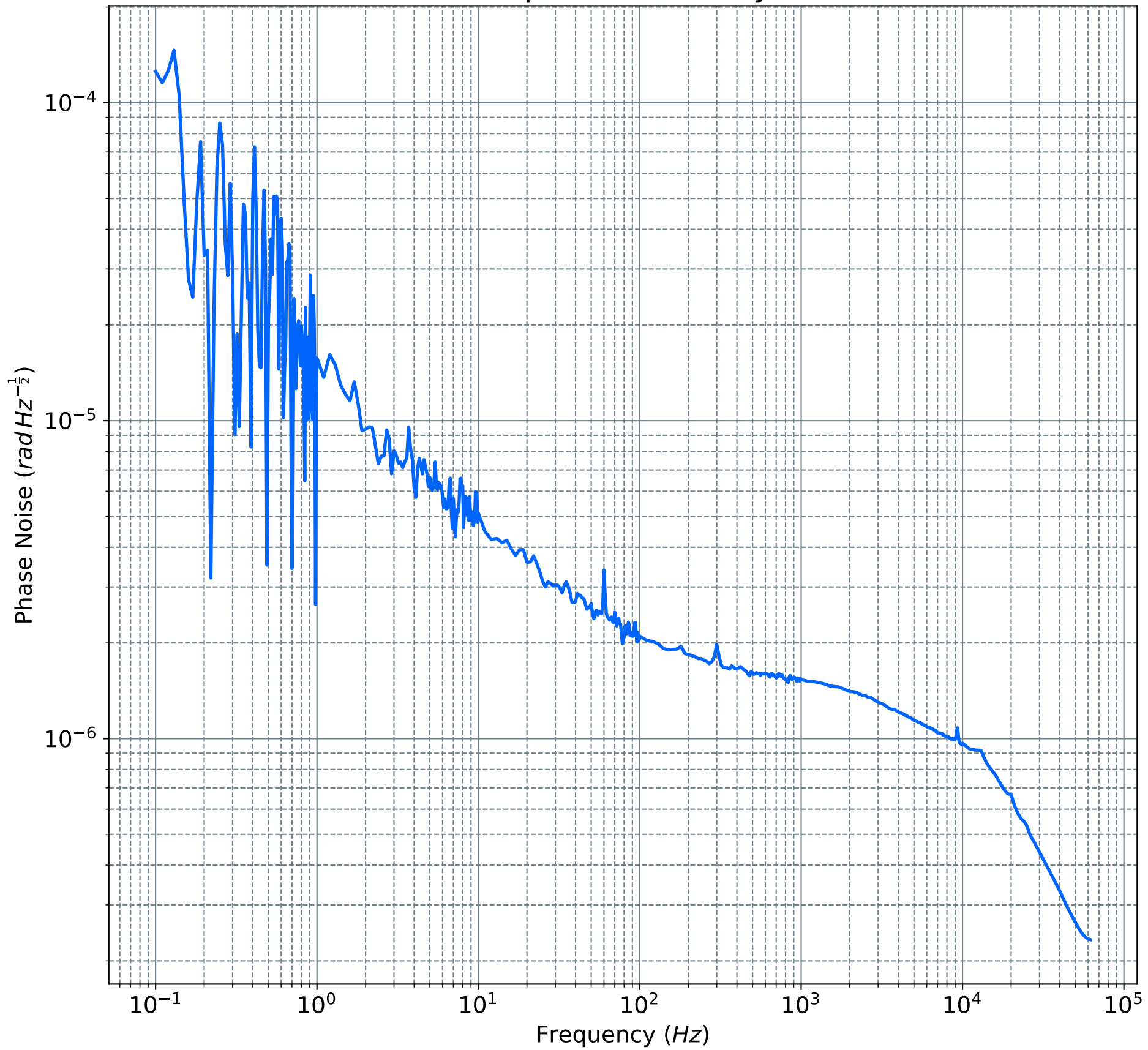
Phase Noise Spectral Density of LO Path
