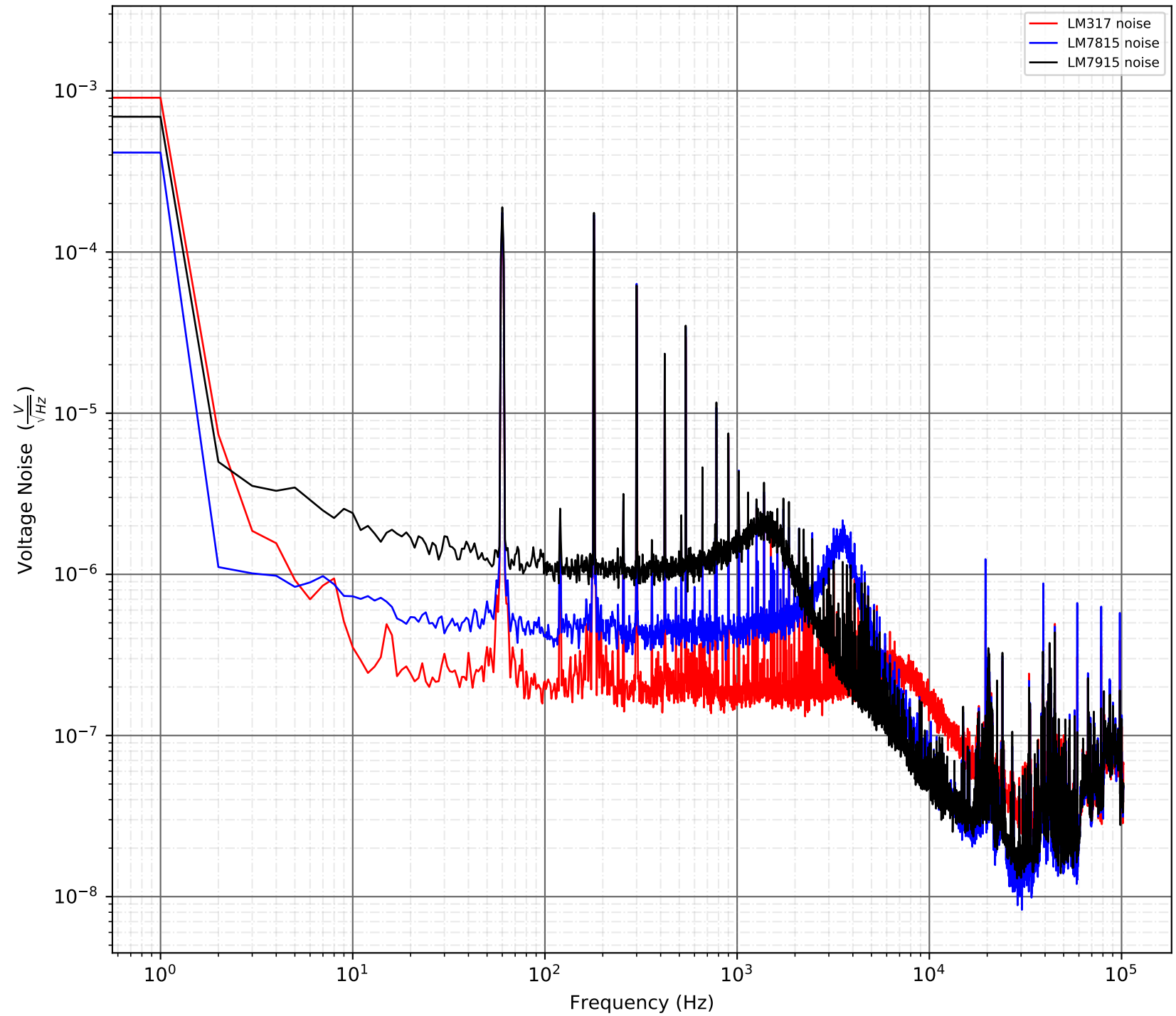
Output Voltage Noise Across Voltage Regulator
