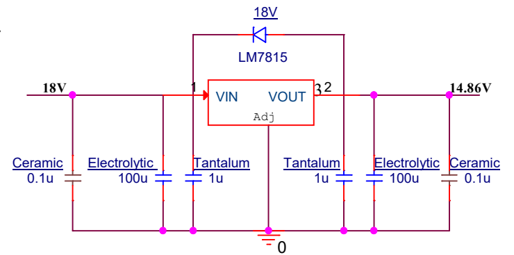
LM7815 regulator
