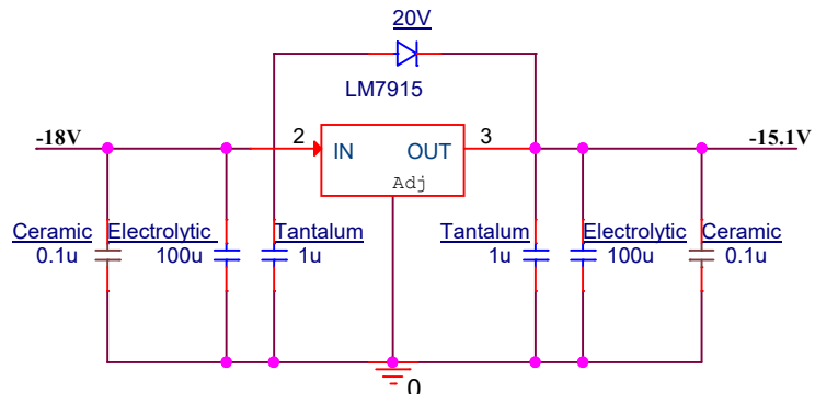
LM7915 regulator
