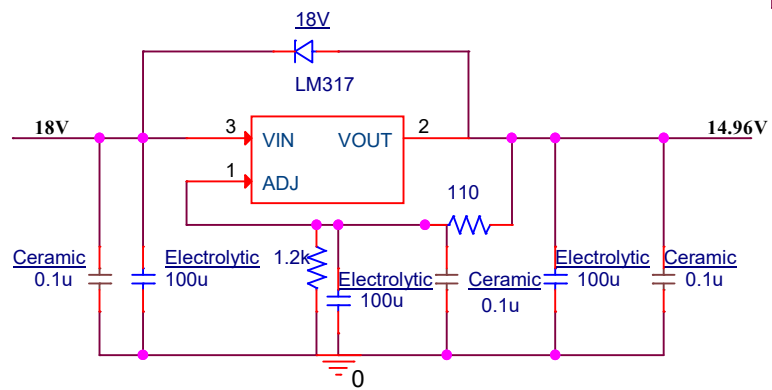
LM317 regulator
