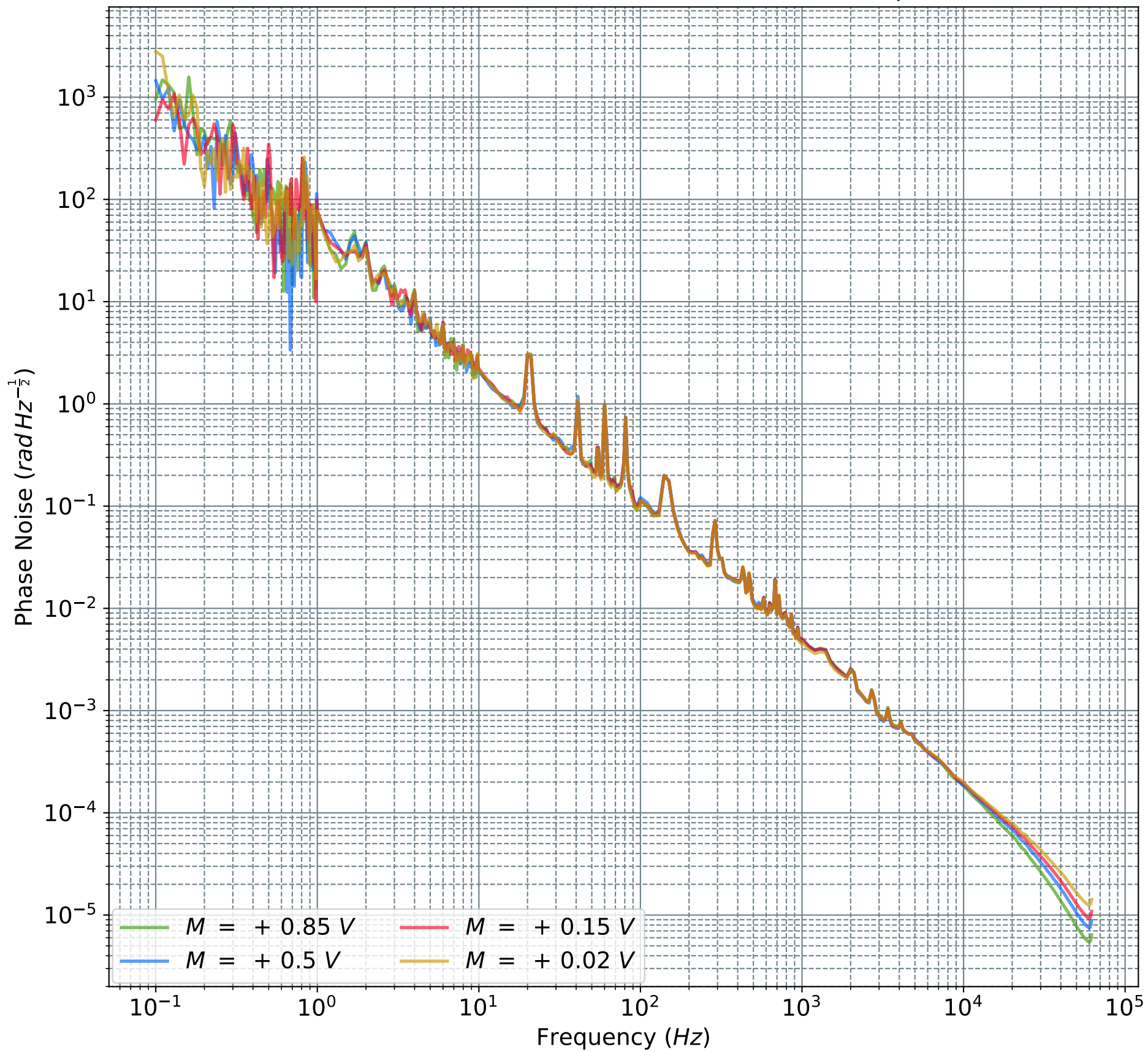
Phase Noise ASD of Brimrose AOM Driver, a VCO.
