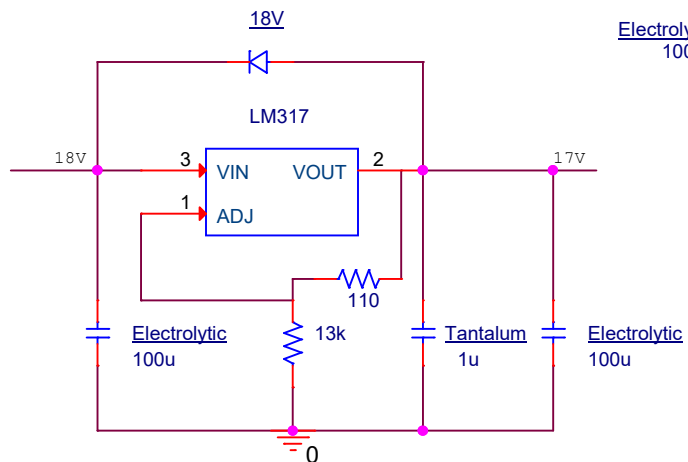
LM317 regulator
