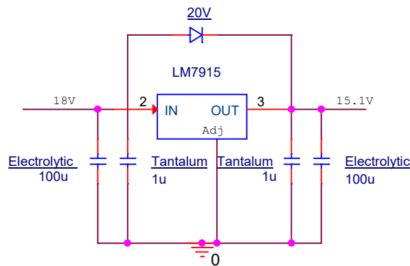
LM7915 regulator
