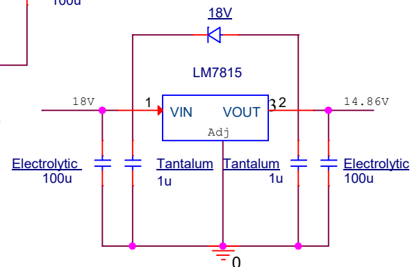
LM7815 regulator
