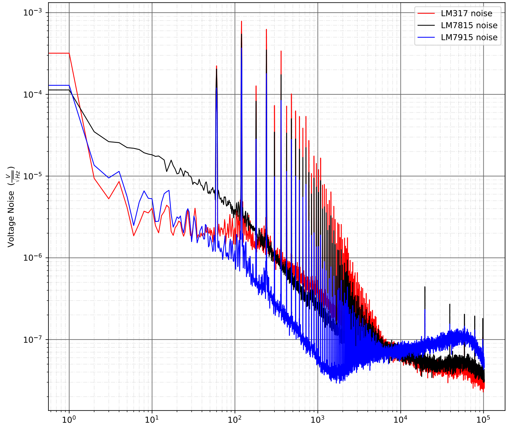
Output Voltage Noise across Voltage Regulator Circuit
