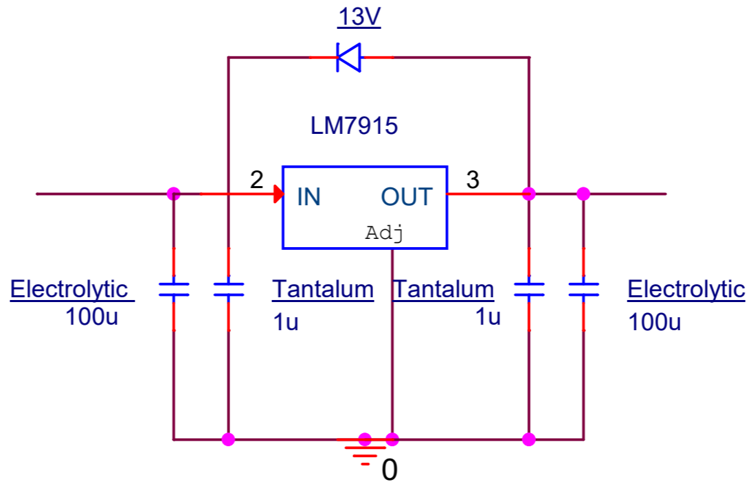
LM7915 regulator
