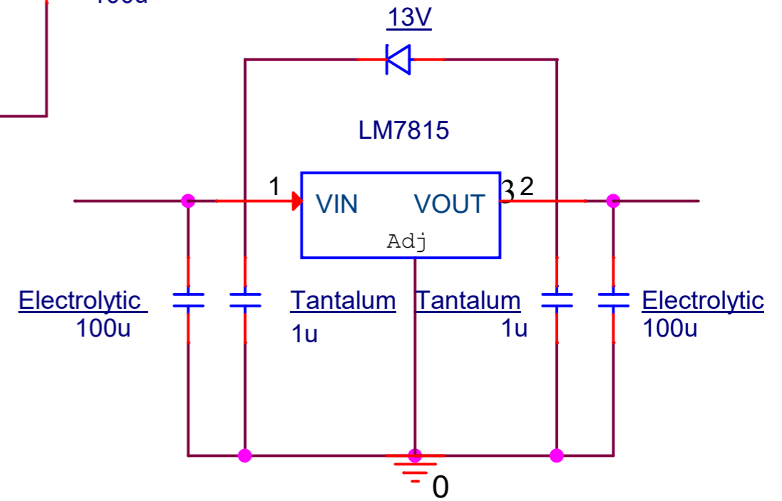
LM7815 regulator
