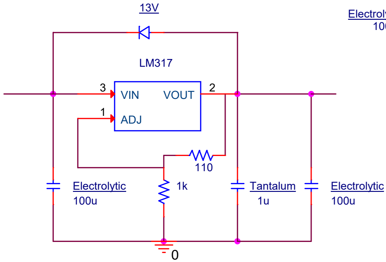
LM317 regulator
