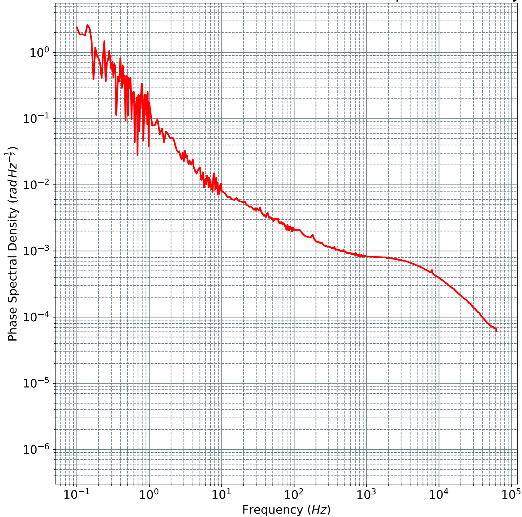
Mach Zehnder IFO Arm: Smooth Phase Spectral Density
