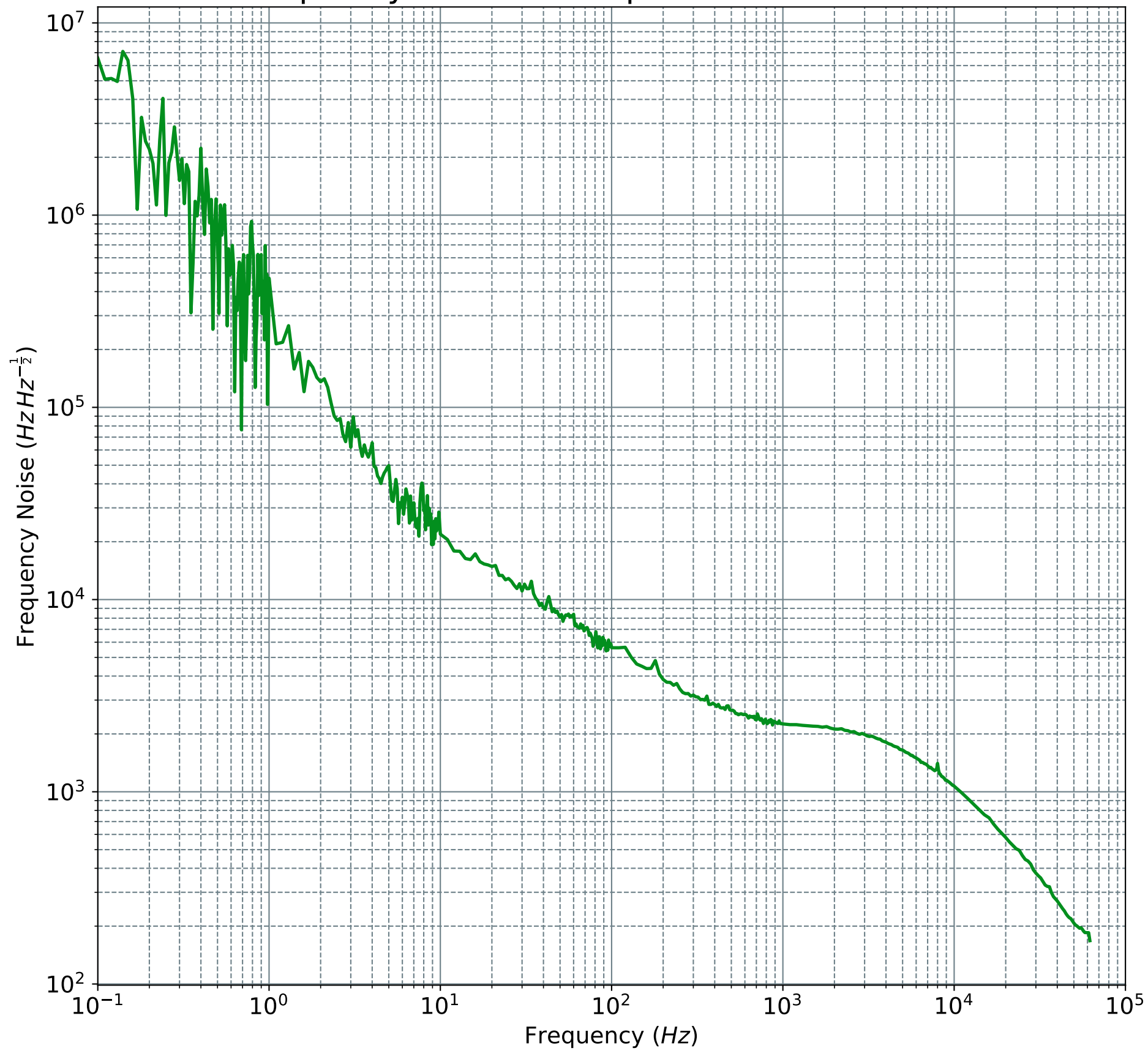
Frequency Noise from 2 \mu m Mach Zehnder IFO
