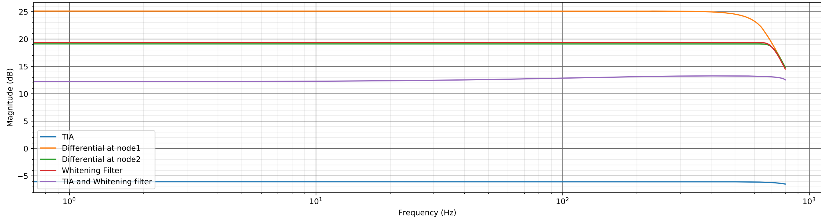
Magnitude Plot
