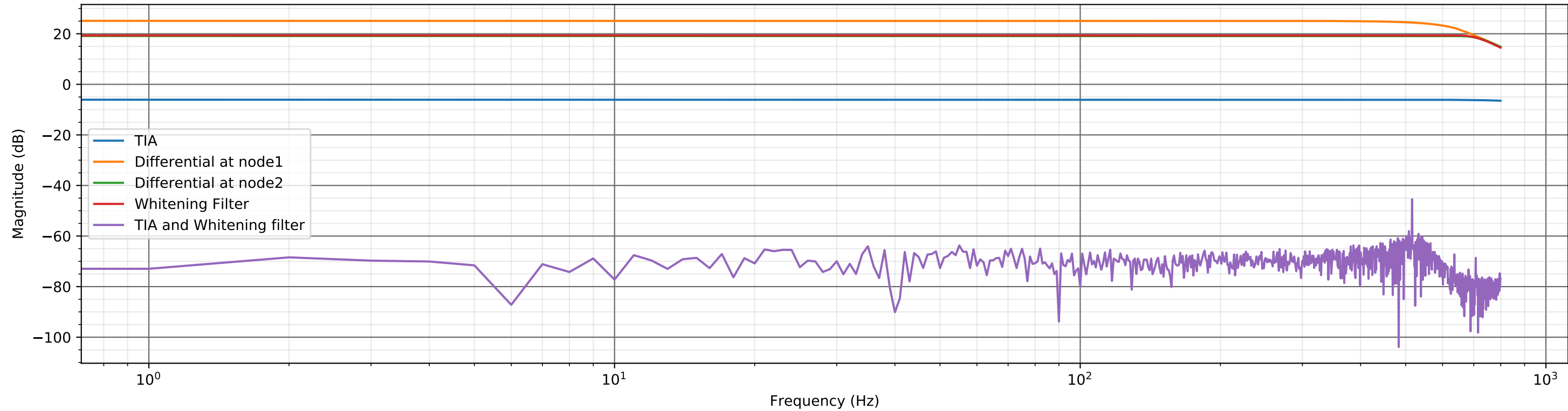
Magnitude Plot
