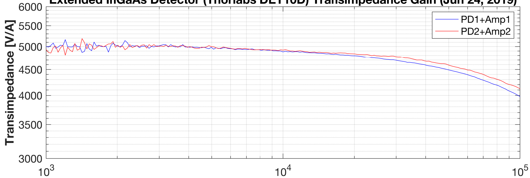
Extended InGaAs Detector (Thorlabs DET10D) Transimpedance Gain (Jun 24, 2019)
