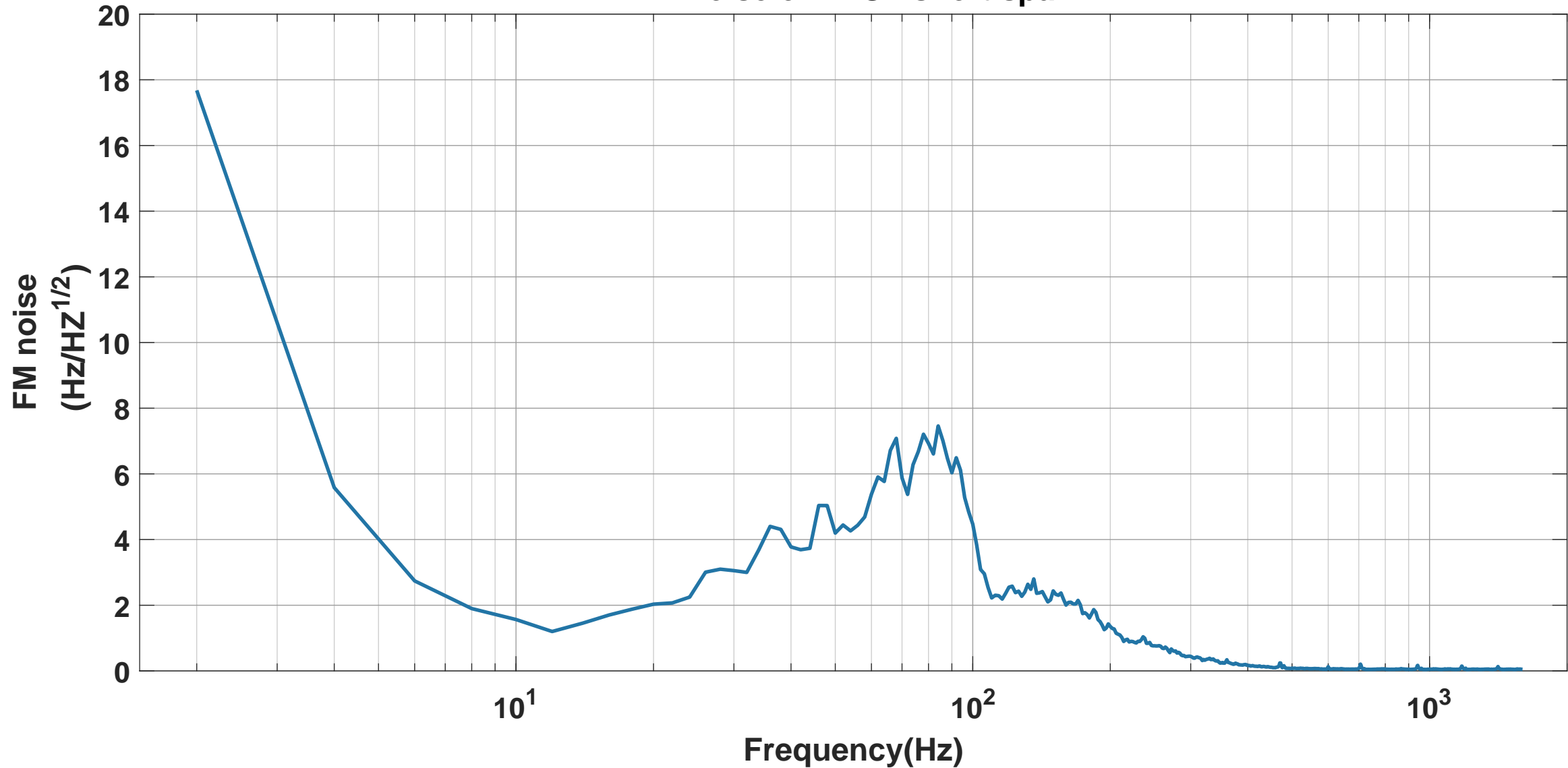
FM noise of AFG - short span
