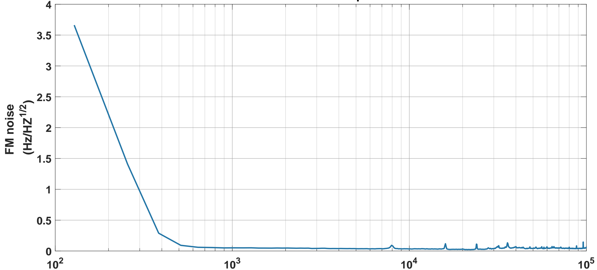
FM noise : Full span
