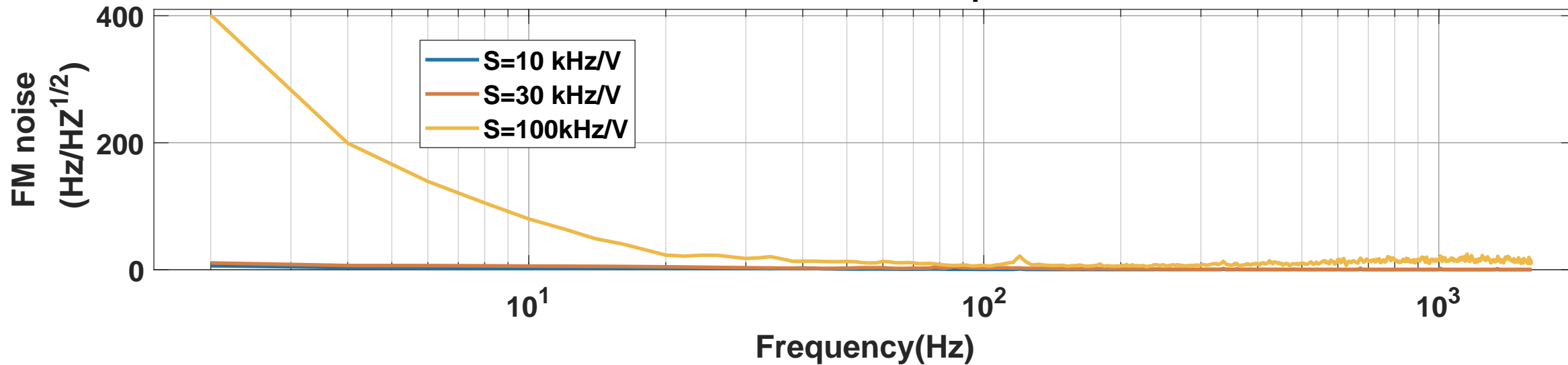
FM noise - short span
