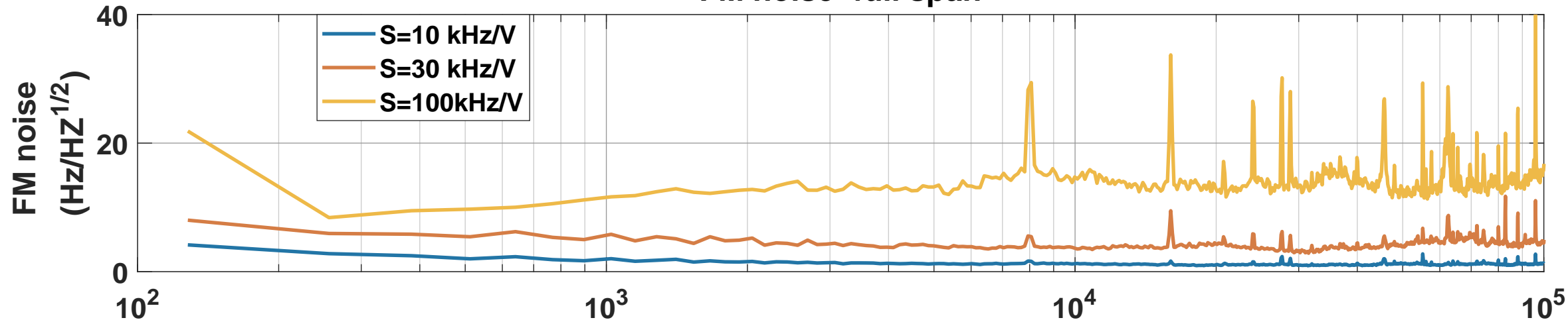
FM noise -full span
