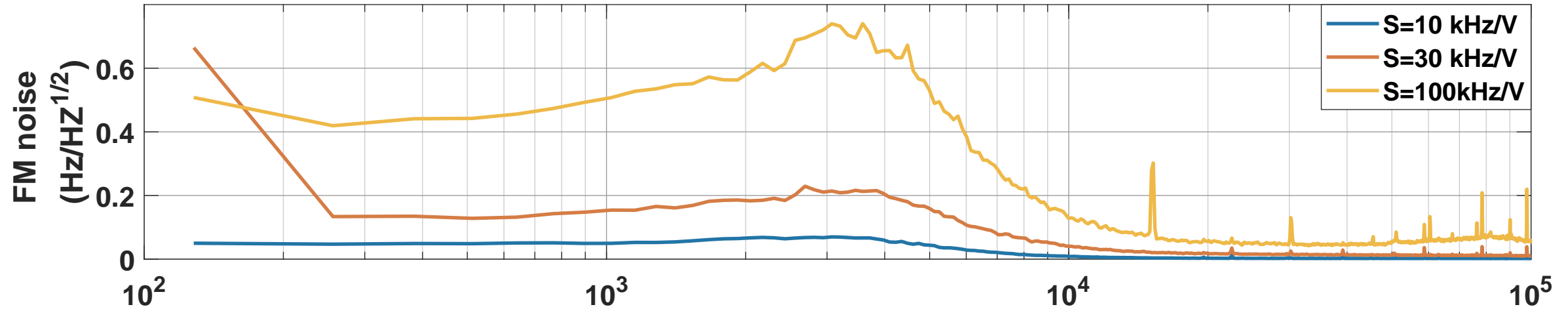
FM noise of AFG -full span
