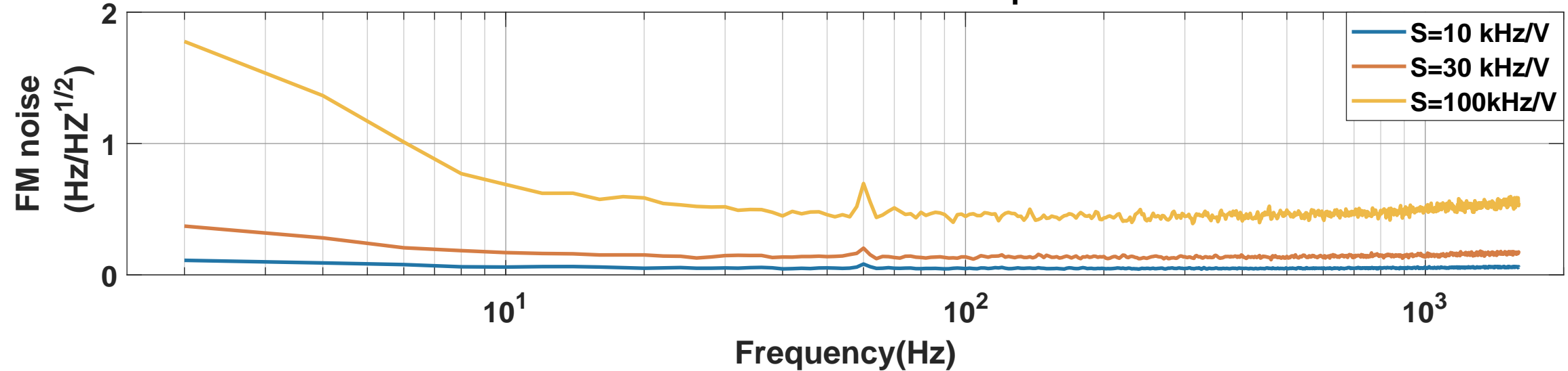
FM noise of AFG - short span
