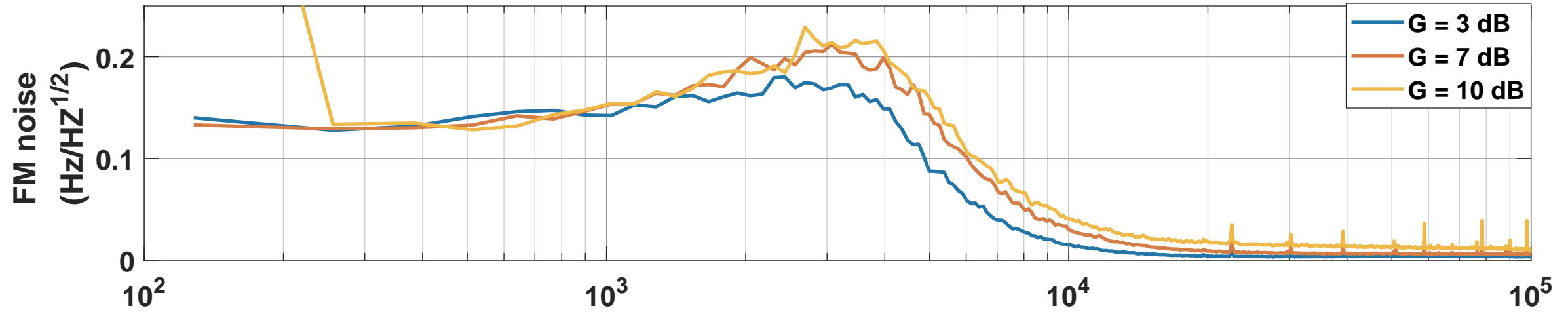
FM noise of AFG -full span
