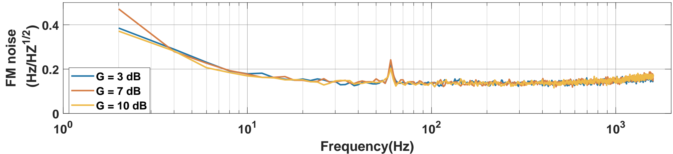
FM noise of AFG - short span
