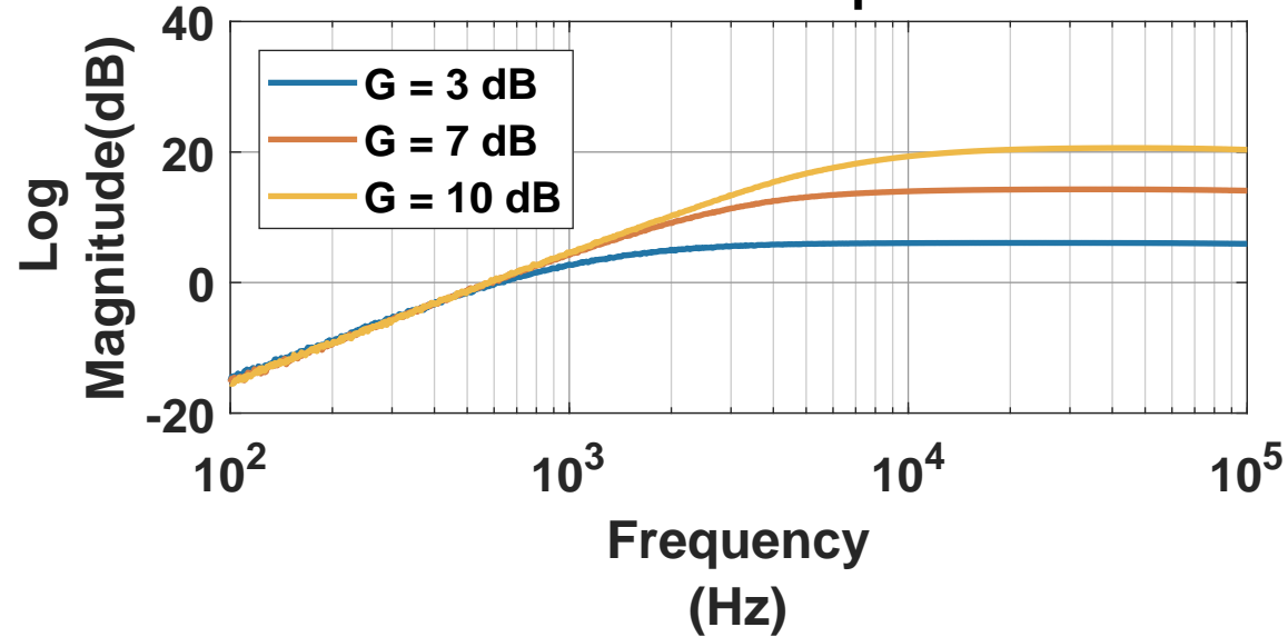
closed loop
