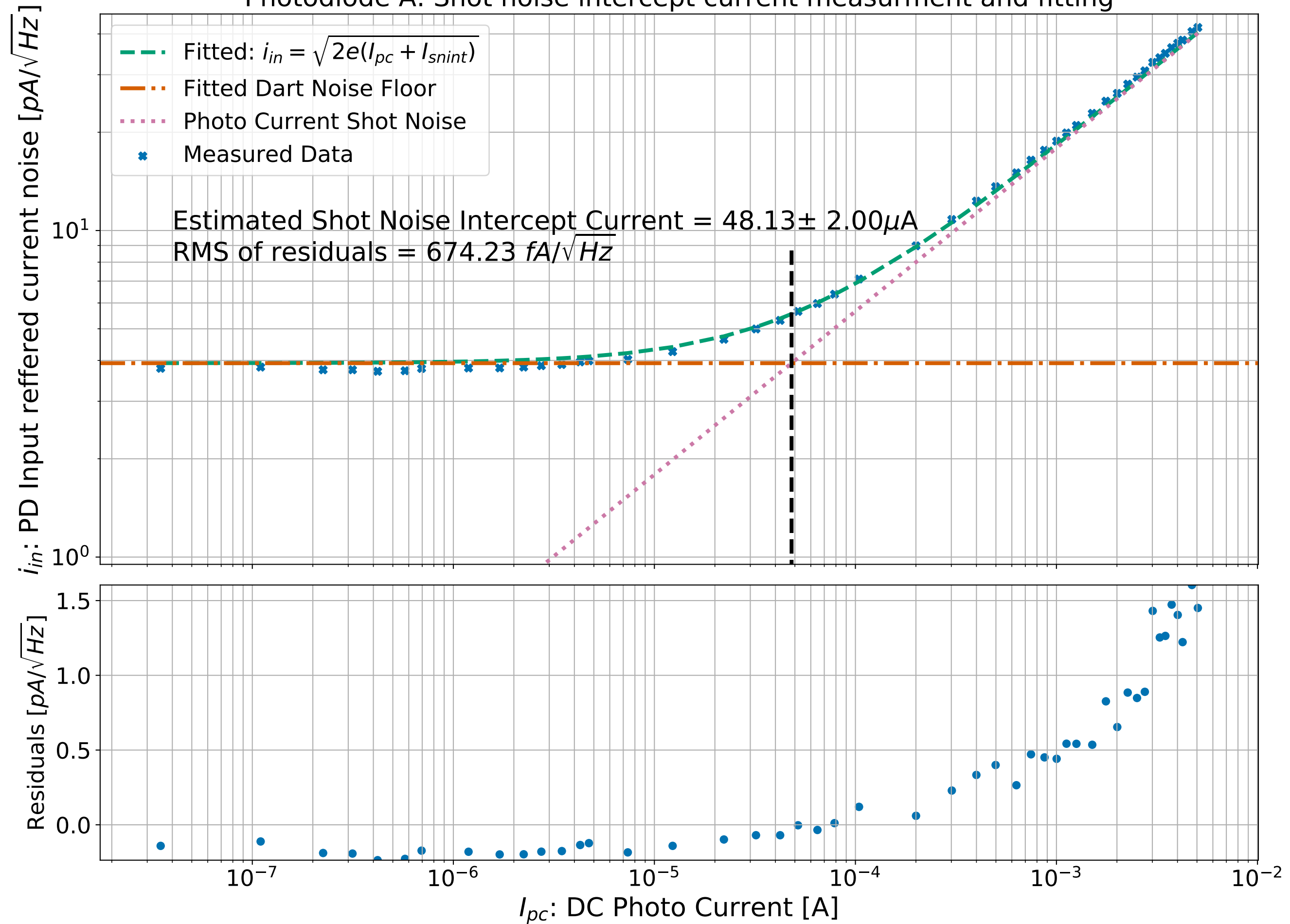
Photodiode A: Shot noise intercept current measurement and fitting
