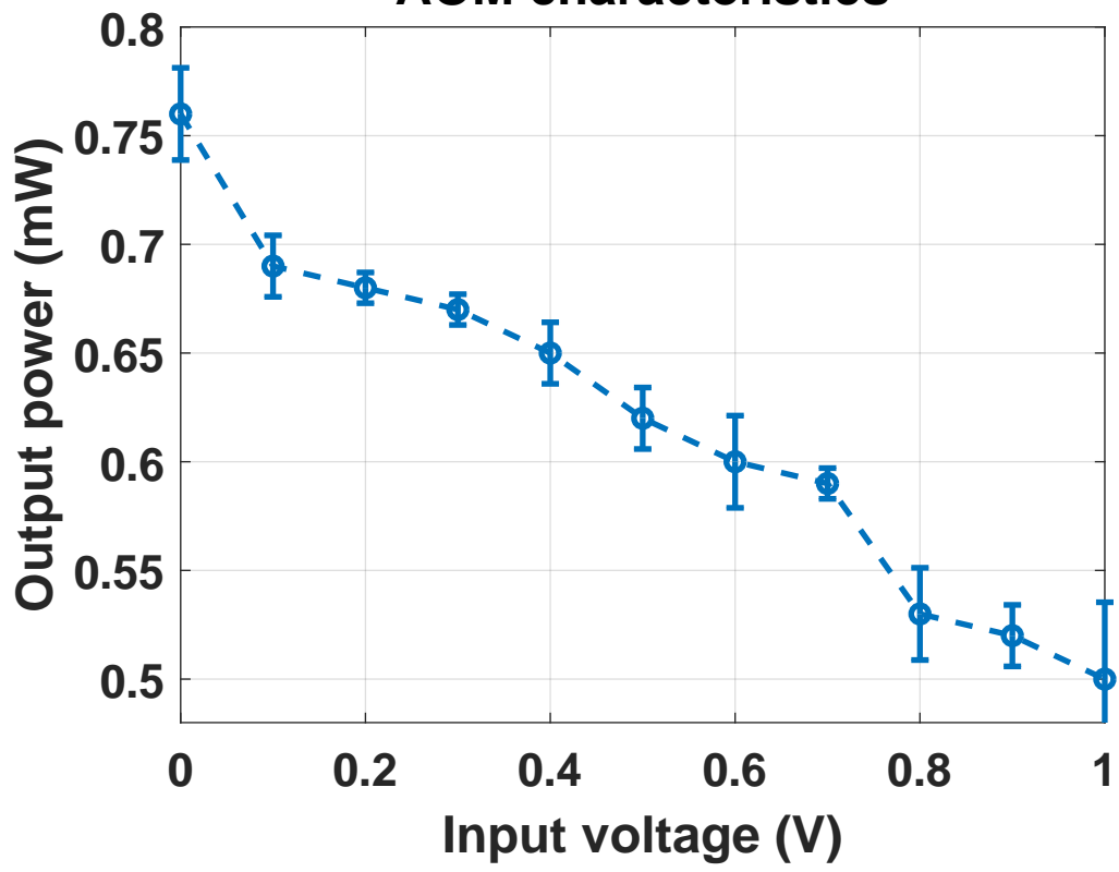
AOM characteristics
